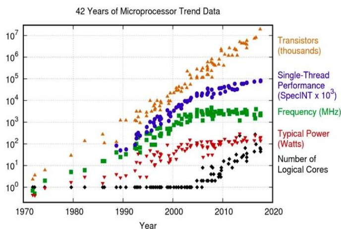
Original data up to the year 2010 collected and plotted by M. Horowitz, F. Labonte, O. Shacham, K. Olukotun, L. Hammond, and C. Batten. New plot and data collected for 2010-2017 by K. Rupp.
