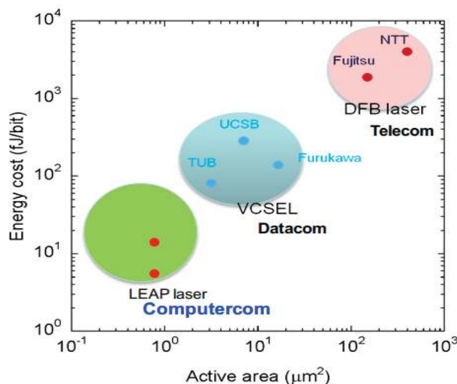
Fig. 11. Energy cost as a function of active region footprint for three different laser technologies (LEAP laser, VCSEL, DFB laser) [169].
