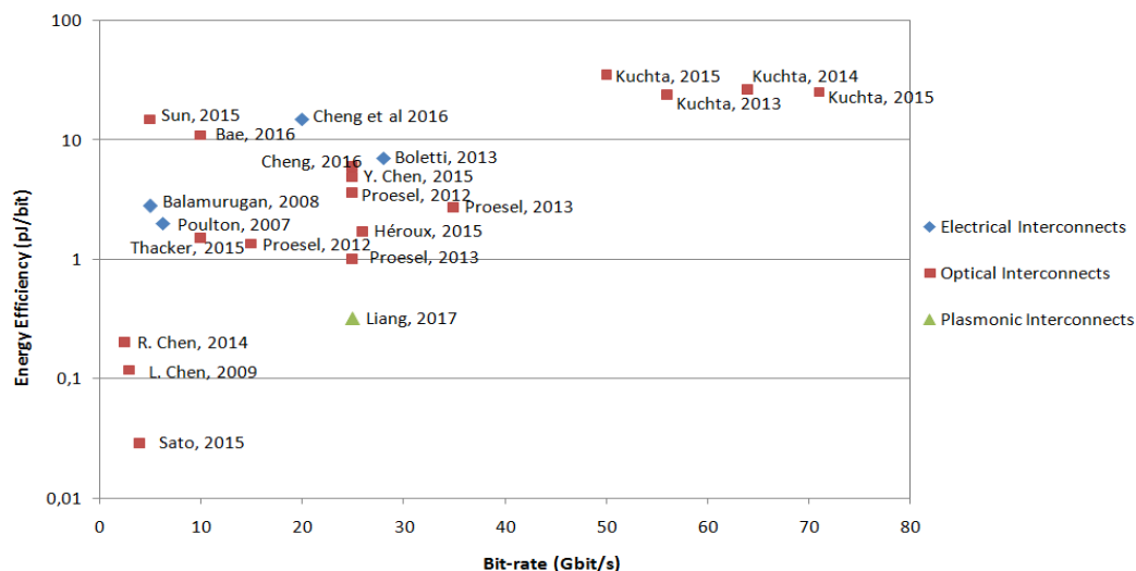
Fig. 9. Total energy dissipation versus bandwidth for conventional electronic, photonic and plasmonic short-reach interconnects (years 2007-2017).
