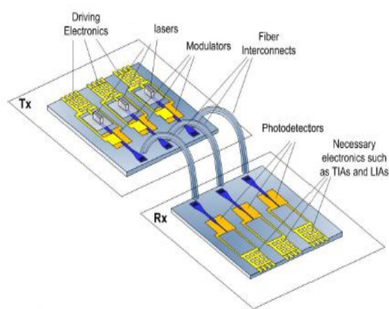
Fig. 10. 2-D typical interconnect structure (Source: Navolchi project [135])
