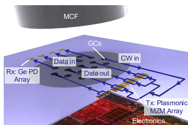
Fig. 6. Compact high-speed optical interconnect scenario: Integrated transceiver consisting of a plasmonic MZM array and a photodiode array. The Tx.: a CW signal of a central laser is coupled to the chip through a multicore fiber (MCF) onto the chip by grating couplers (GCs). The light is then distributed to the integrated plasmonic MZMs to encode a parallel data stream. After encoding, the signals are coupled out via separate cores of the MCF. Rx side: PDs receive the signals stemming from different cores of the MCF. The electronic contacts of the devices may be realized through vias from the bottom of the chip [102].
