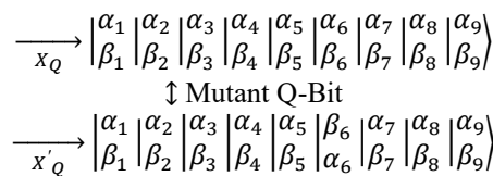
Figure 13: Example of a quantum bit mutation operator
