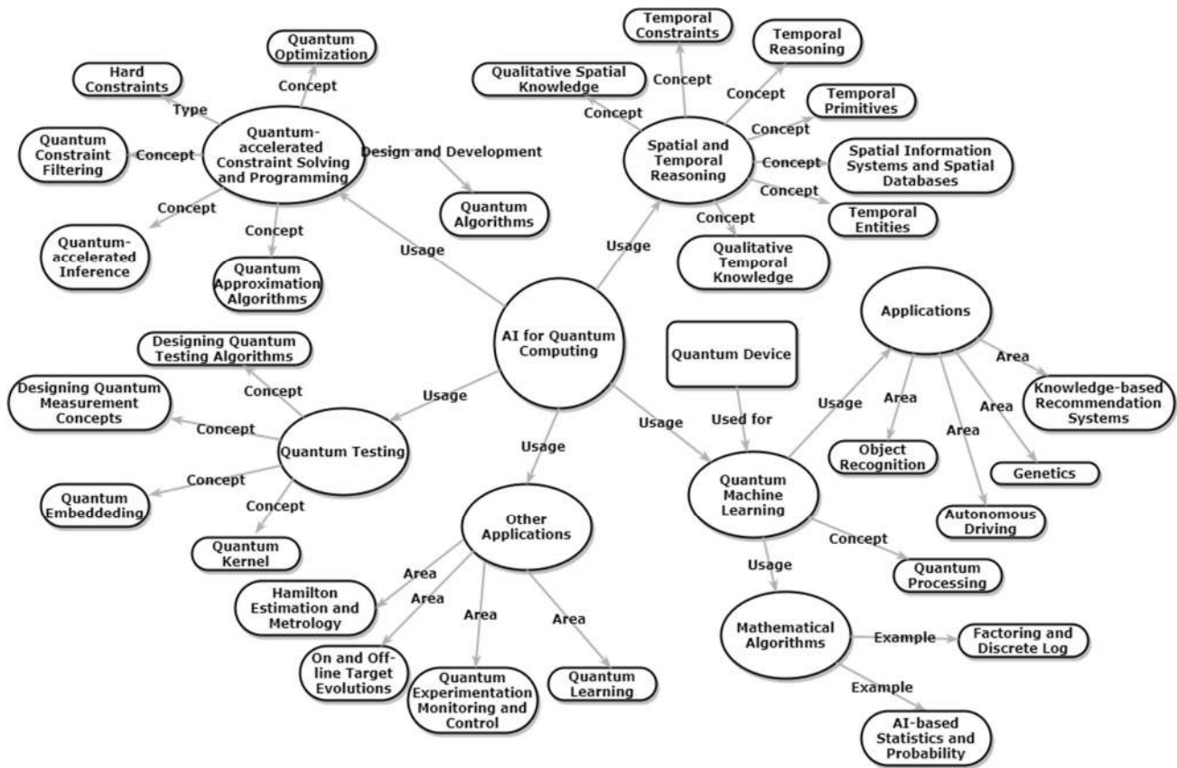
Figure 7: AI for Quantum Computing
