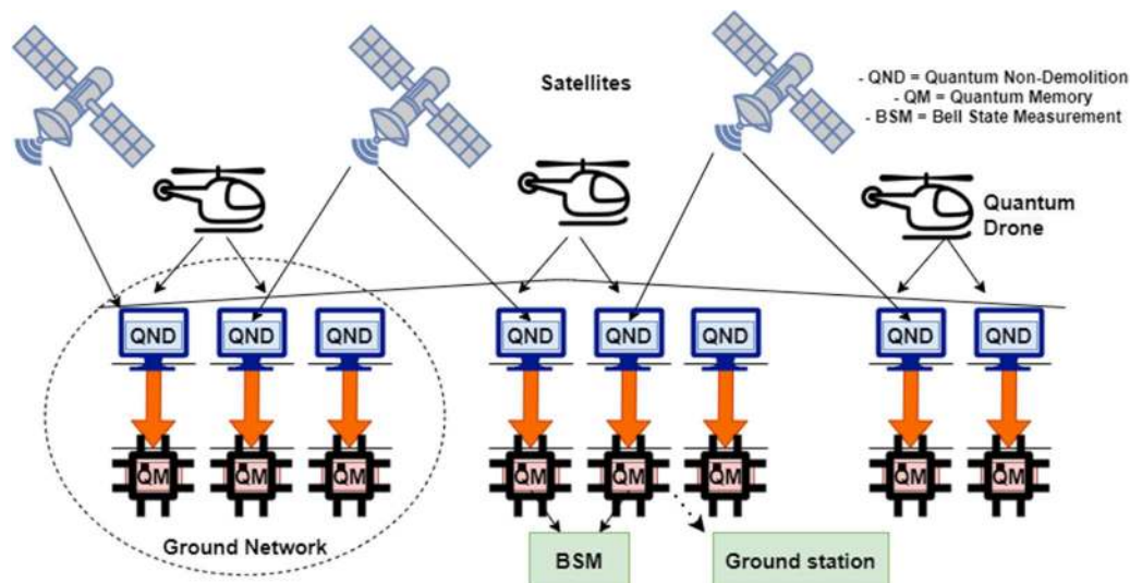
Figure 10: Architecture of a Q-Repeater
