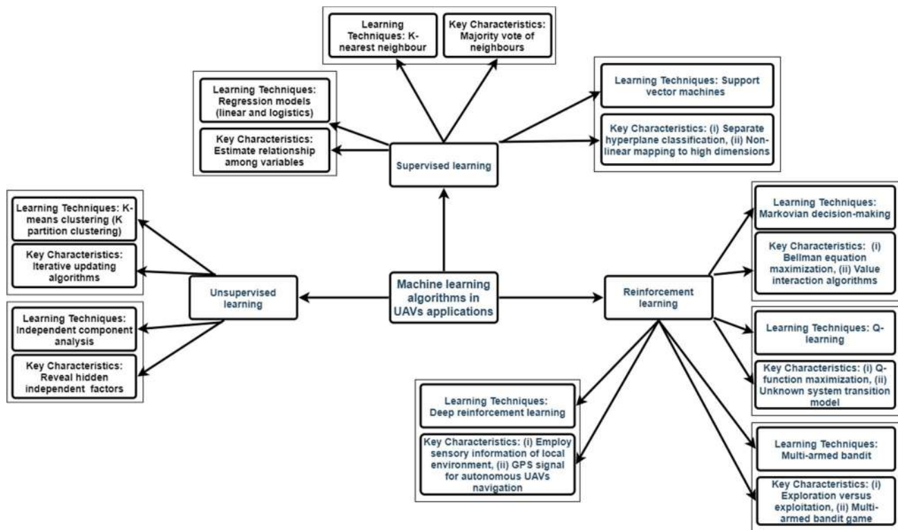
Figure 6: Machine learning algorithms in UAVs applications [132].
