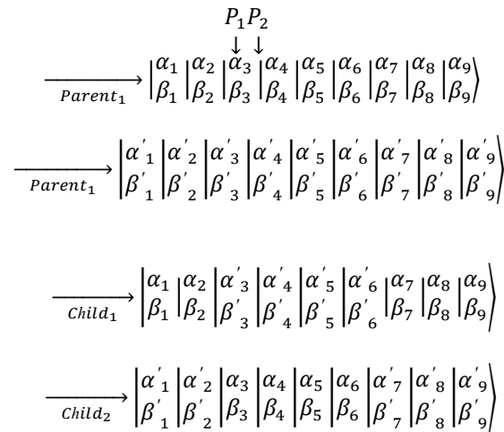
Figure 12: Example of Two Point Quantum Crossover
