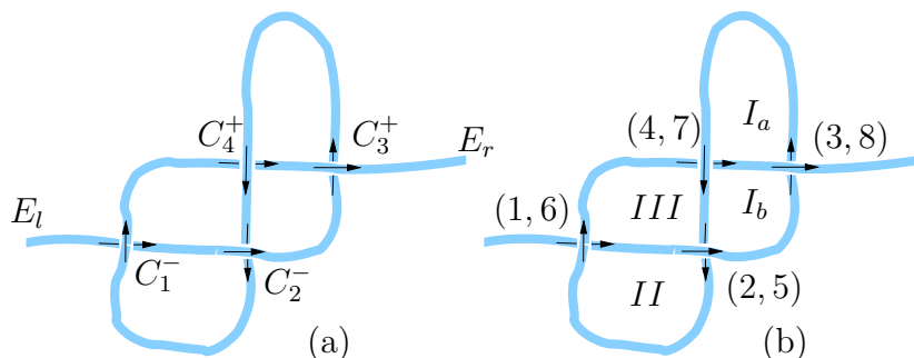
Figure 2: (a) Sequence of crossings representing the state of the rope: E_l - C_1^{l-} - C_2^{u-} - C_3^{l+} - C_4^{u+} - C_2^{l-} - C_1^{u-} - C_4^{l+} - C_3^{u+} - E_r . The first two crossings are left-handed helical (labelled with a minus sign) and the other two are right-handed helical (plus label). The labels u and l refer to the upper and lower part of the crossing, respectively. (b) An alternative representation, used in [43]. The numbering of the loops is conditioned by the forming sequence, which in this case is (2, 5), (1, 6), (4, 7), (3, 8) (this corresponds to reversing the upper sequence shown later in Figure 9), note that the last step pierces loop I in two loops I_a and I_b .
