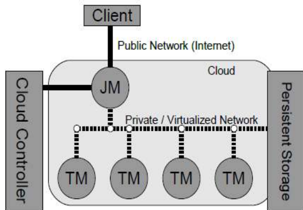
Fig. 3 Design Architecture of Nephelē Framework [4]
