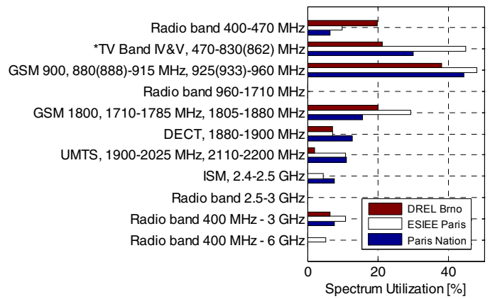
Figure 7. Comparative summary on regional spectrum utilization.
