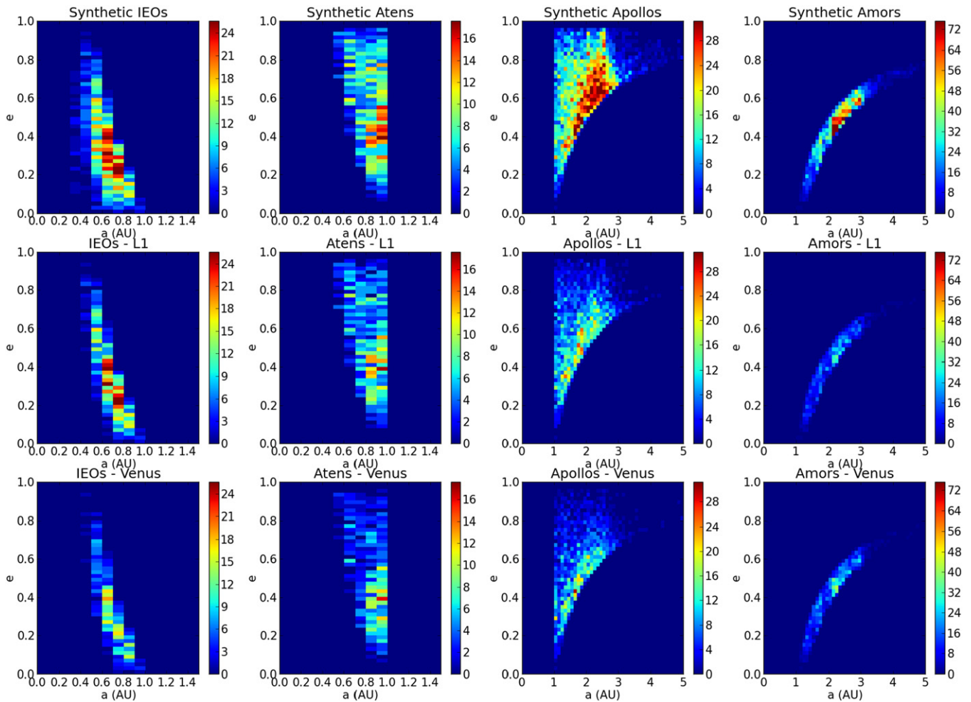
Figure 15. Distribution of semimajor axis vs. eccentricity for one of the 25 input synthetic NEA subpopulations (top row), compared with the distributions of objects detected with >22 days observational arcs that were found by the L1 survey (middle row) and the Venus-trailing survey (bottom row) after 5 yr.
