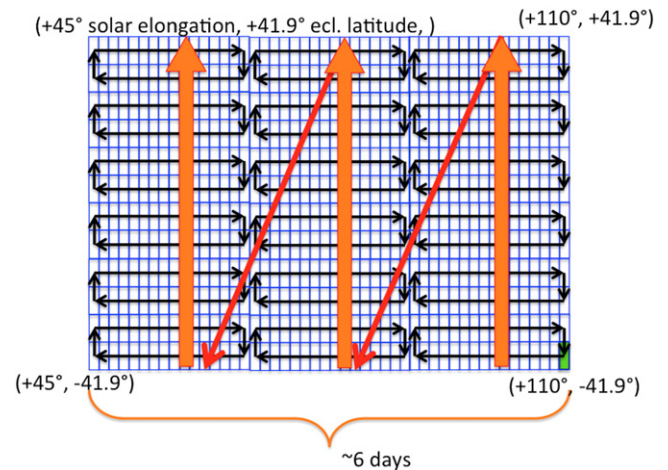
Figure 5. Survey pattern over \sim 6 days for the L1 survey. Green indicates the starting field.
