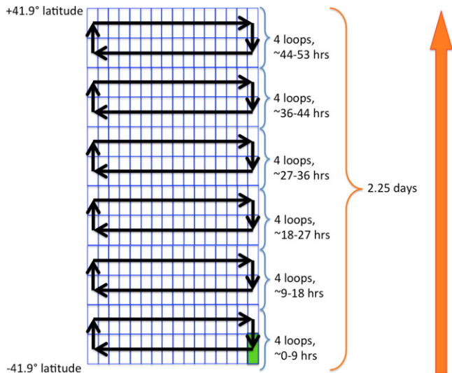
Figure 4. Loop pattern repeated, increasing in ecliptic latitude, over \sim 2.25 days. The green rectangle indicates the starting position.
