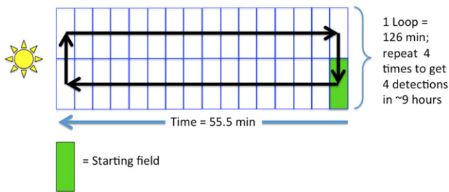
Figure 3. Basic element of the survey cadence, a “quad,” which consists of four observations taken over \sim 9 hr. The green rectangle indicates the starting position.
