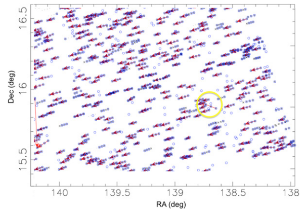
Figure 11. Set of example candidate tracklets with four or more detections generated for one patch by XMOPS (red arrows indicate the start and end points of the tracklets). Empty blue “o” marks show the simulated detections that match the position, time, magnitude, and coverage criteria and were not identified as stationary sources. Black “x” marks show the expected, true known solar system objects that match the time/position window as well as the magnitude and coverage thresholds. An “x” without an “o” is a true, detectable solar system object that did not survive stationary object rejection, and an “o” without an “x” is a stationary source that survived stationary object rejection. Any “x” or “o” that is not covered by a red arrow was not linked into a tracklet. All but two of the red arrows represent Main Belt asteroids; the sole NEA in the frame is highlighted by the yellow circle. An example of an erroneously cross-linked tracklet is shown by the nearly vertical red arrow on the extreme left.
