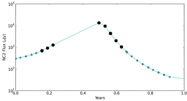
Figure 20. Sample observations of a synthetic Apollo detected 44 times over ~6 months (black circles; each circle contains ~3–13 individual observations). The cyan points show the flux of the object when it passes through the L1 survey’s field of view but is not bright enough to be detected.
