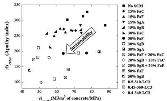
Fig. 8 Decision framework based on the A-index and energy intensity for chloride exposure
