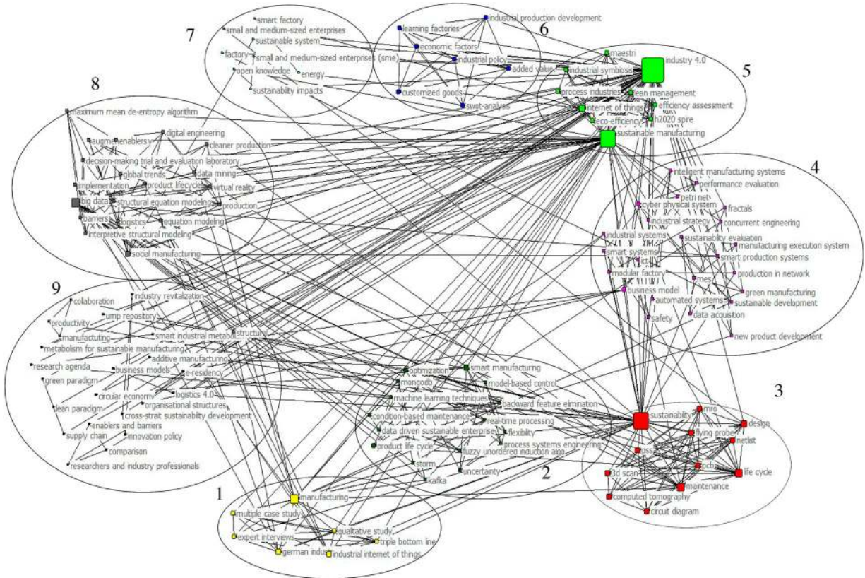
Figure 5. Keywords' network.
