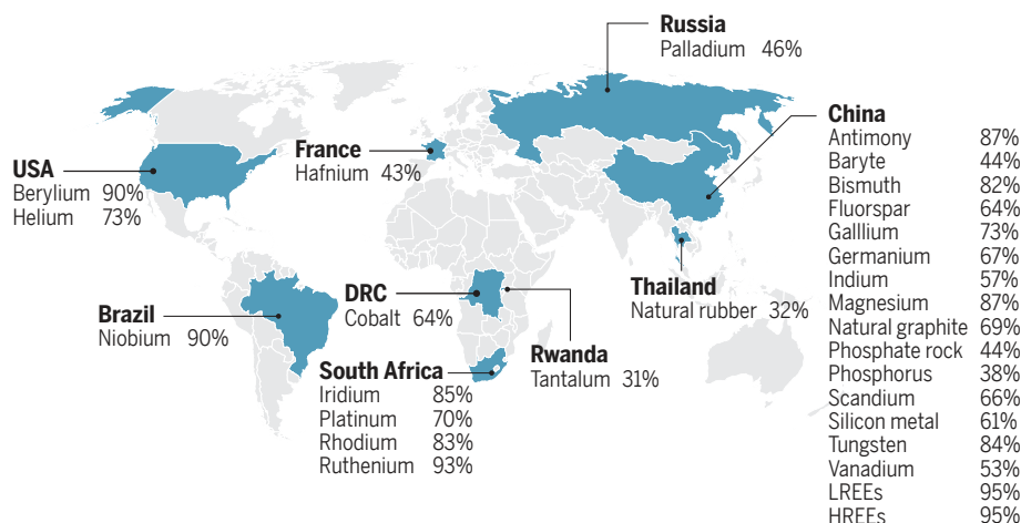
Modified from European Commission. 2017. Third list of critical raw materials for the EU of 2017. Available at https://ec.europa.eu/growth/sectors/raw-materials/specific-interest/critical_en .
