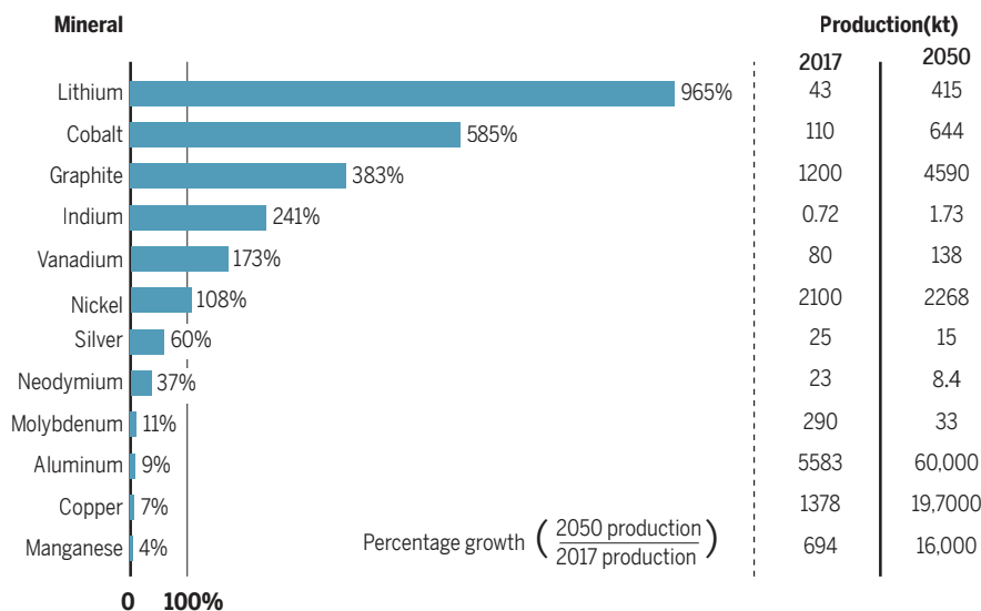
All production data reflect annual production. 2017 data reflect annual production for all uses. 2050 data reflect estimated production for only LCET uses. Modified from World Bank. 2018. Climate-Smart Mining: Minerals for Climate Action. Available at https://www.worldbank.org/en/topic/extractiveindustries/brief/climate-smart-mining-minerals-for-climate-action .
