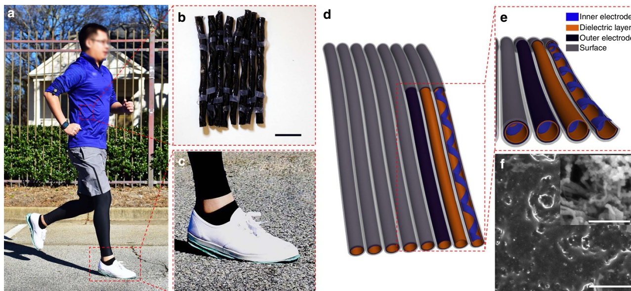
Figure 1 | Overview of the TENG. (a) TENG woven into a coat and assembled under shoes to drive wearable electronics such as an electronic watch and a fitness tracker. (b) Photograph showing TENG tubes in diameter of 2–3 mm woven into textile. (c) Photograph showing TENG-tubes fixed under a shoe. (d) Structure sketch of the TENG tubes. (e) Enlarged view of the TENG structure. (f) SEM image of the triboelectric electrode surface. The inset shows the SEM image of the carbon black/CNTs mixture, which is the conductive ingredient of the inner and outer electrodes. Scale bars in b , f and the inset in f are 1 cm, 5 \mu\text{m} and 500 nm, respectively.
