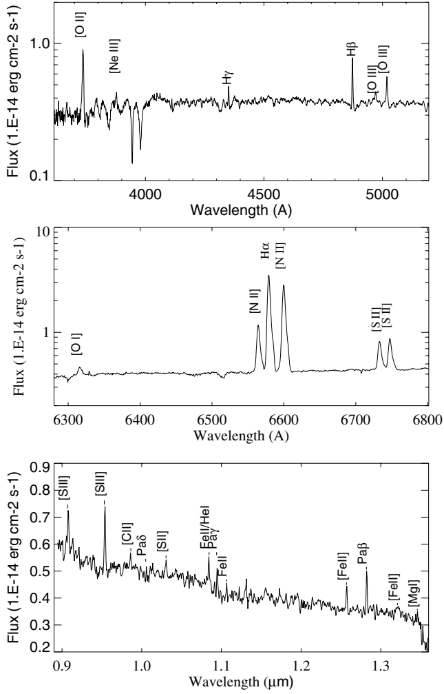
Fig. 6. Optical spectrum observed with TWIN in Calar Alto observatory ( top and middle panels ) and near-infrared spectrum observed with LIRIS in El Roque de los Muchachos Observatory ( bottom panel ). The optical and near-infrared spectra were taken 1 week apart from each other, and one month after the Suzaku observation. The optical spectra are in arbitrary units since the absolute calibration could not be done (see text).
