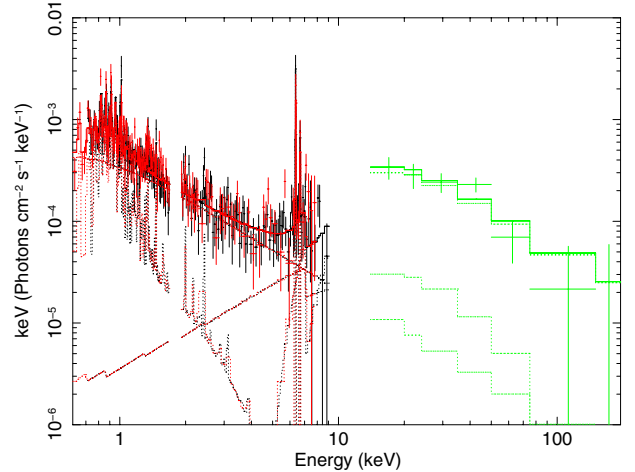
Fig. 5. Best fit to the Suzaku /XIS (red and black) and Swift/BAT (green) spectra.
