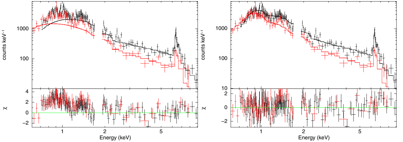
Fig. 3. ( Left ): Extrapolation of the 2–9 keV XIS/ Suzaku best-fit model ( Model C ) to lower energies. ( Right ): Final fit ( top panel ) and residuals ( bottom panel ) to the XIS/ Suzaku data using Model E . See Table 1 and text for an explanation on the components used in each model.
