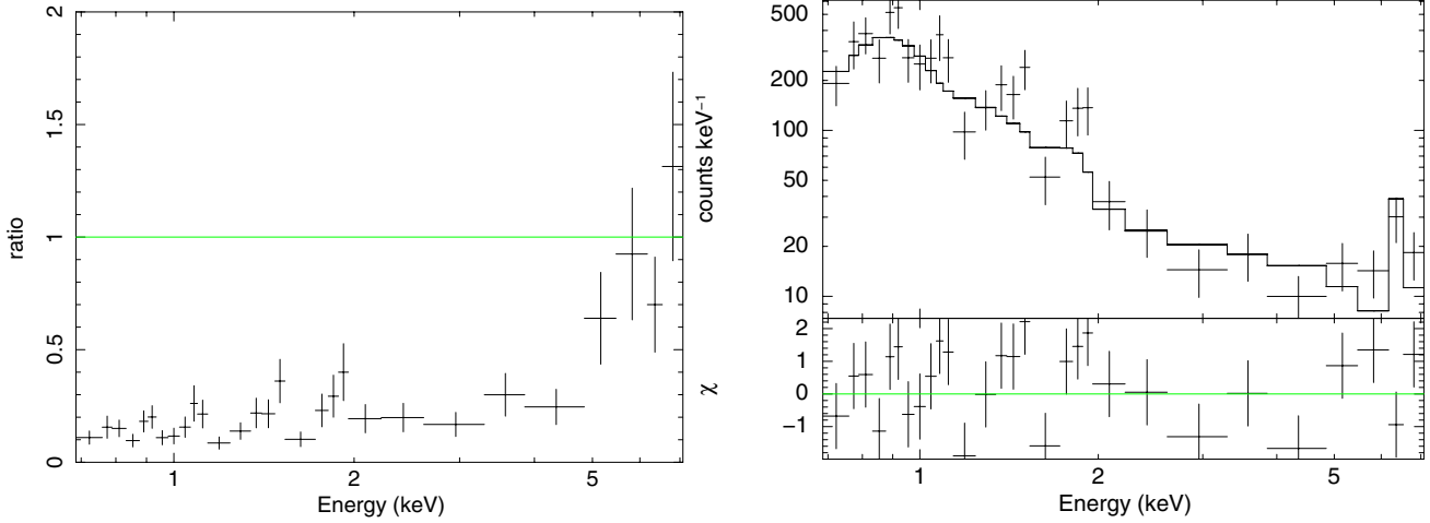
Fig. 4. (Left): ratio between the ACIS/ Chandra and the XIS/ Suzaku data best-fit Model E . (Right): Chandra best-fit (top panel) and residuals (bottom panel) using Model E and varying the normalisation of the power law and the thermal components by the same amount.
