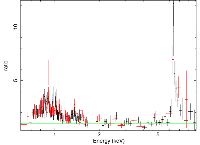
Fig. 1. Ratio between XIS/ Suzaku data and a power-law model fitted to the 2–6 keV band. Black (dark) points indicate the XIS-0+3 spectrum and red (light) points the XIS-1 spectrum.
