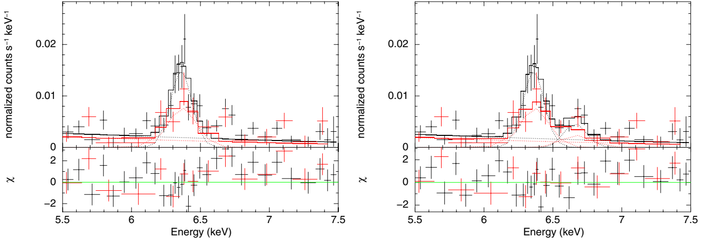
Fig. 2. Best-fit ( top panels ) and residual ( bottom panels ) plots of Suzaku /XIS data for Model A ( left ) and Model B ( right ) around the Fe emission region (black and red points as in Fig. 1). The dotted lines indicate the various model components.
