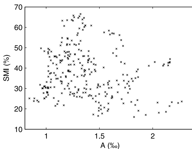
Figure 4. Scatterplot of annual amplitudes (A) against stratigraphic melt index (SMI) using 15 year moving averages (1700–1970). There is no simple relationship between melt and amplitudes. Scatter increases when using 5 year averages.
