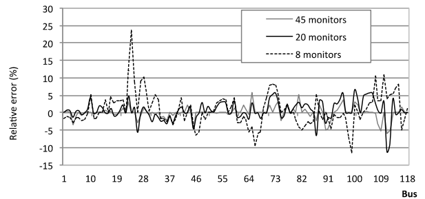
Fig. 8: Relative error in the estimation of the number of sags with remaining voltage below 0.9 p.u.
