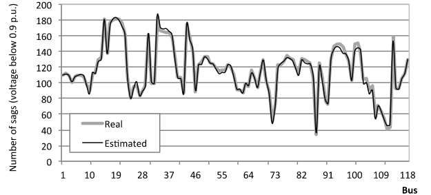
Fig. 2: Actual and estimated number of voltage sags with residual voltage below 0.9 p.u. at the IEEE 118 test system buses.
