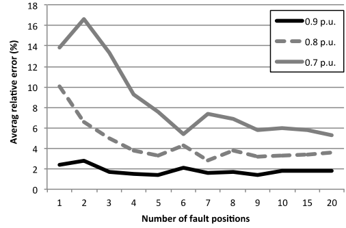
Fig. 7: Average RE_j (%) in the estimation of the number of sags by considering different numbers of fault positions.
