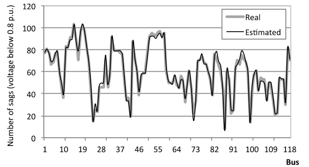
Fig. 3: Actual and estimated number of voltage sags with residual voltage below 0.8 p.u. at the IEEE 118 test system buses.
