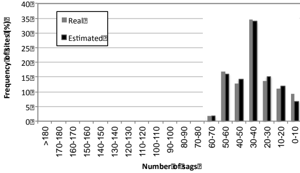
Fig. 6: Frequency of sites having a certain number of sags with remaining voltage below 0.7 p.u.
