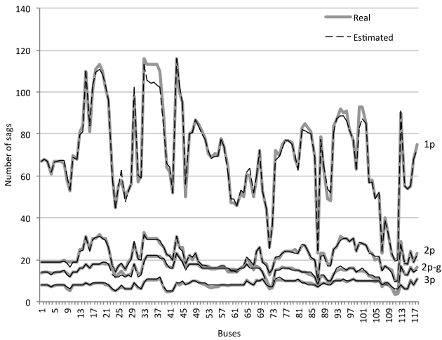
Fig. 9: Actual and estimated number of voltage sags with residual voltage below 0.9 p.u. for different types of fault.
