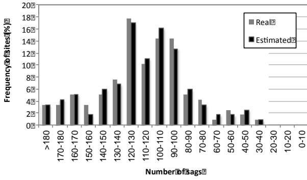
Fig. 5: Frequency of sites having a certain number of sags with remaining voltage below 0.9 p.u.
