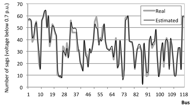
Fig. 4: Actual and estimated number of voltage sags with residual voltage below 0.7 p.u. at the IEEE 118 test system buses.
