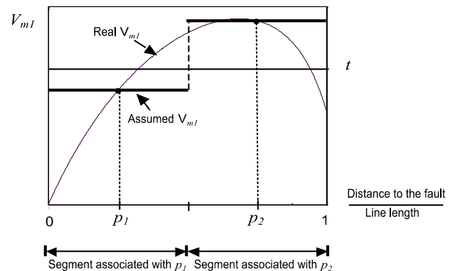
Fig. 1: Real and assumed remaining voltage.
