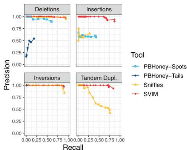
Fig. 4. Comparison of SV detection performance on a 6× coverage homozygous simulated dataset. SVIM consistently yielded better recall (x-axis) and precision (y-axis) than the other tools for the recovery of INs and tandem duplications. For the recovery of deletions and inversions, Sniffles reached the same recall as SVIM. The different points for each tool represent multiple settings of the tools' most important parameters (see Section 2.5). PBHoney-Spots only detects deletions and INs and PBHoney-Tails does not detect duplications. Recall and precision were calculated using a required reciprocal overlap of 50% between variant calls and the original simulated variants
