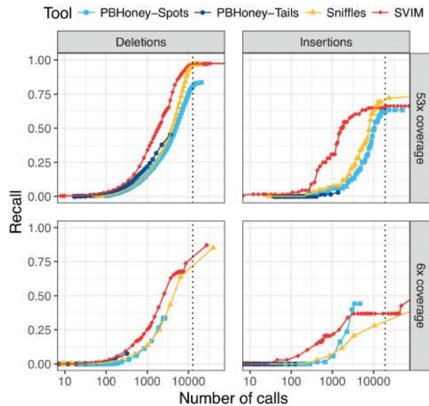
Fig. 5. Comparison of recall on a 53× coverage public PacBio dataset and a 6× coverage subset with 2676 high-confidence deletion and 68 insertion calls. For each tool and different thresholds, the number of SV calls with score above the threshold (log-scale) is plotted against the recall. The upper and lower panels show performance on the full dataset and a randomly sampled 6× coverage subset of the data, respectively. SVIM reached the same recall with fewer calls than other tools. The vertical dotted lines denote the average number of deletions and insertions to expect in an individual as recently reported using a de-novo assembly approach (Chaisson et al. , 2018). Recall was calculated using a required reciprocal overlap of 50% (deletion calls) and 1% (insertion calls), respectively, between variant calls and the gold standard variants
