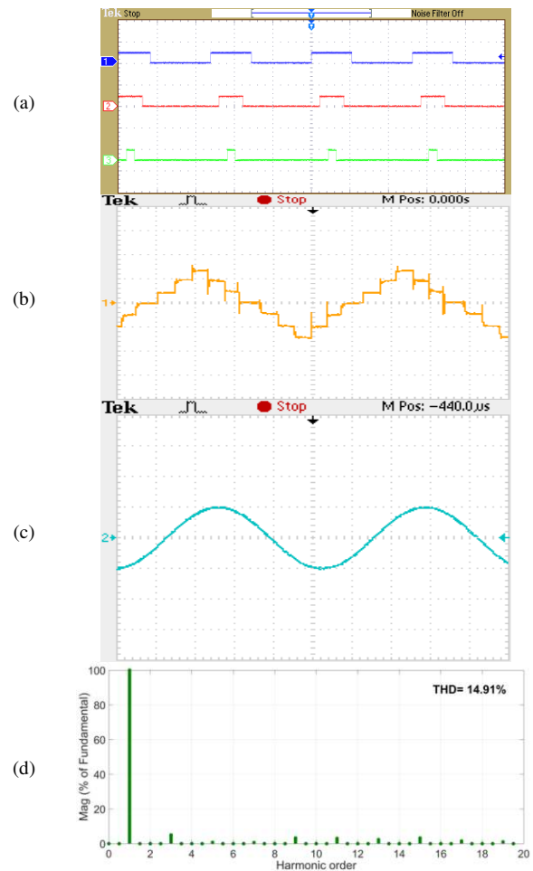
Fig. 9. Experimental results for 7-level CHB MLI: (a) PWM signals for switches T_1 , T_5 , and T_9 (y-axis 20V/div, x-axis 2ms/div), (b) Output voltage waveform (y-axis 50V/div, x-axis 1ms/div), (c) Output current waveform (y-axis 1A/div, x-axis 1ms/div), (d) FFT analysis of load voltage
