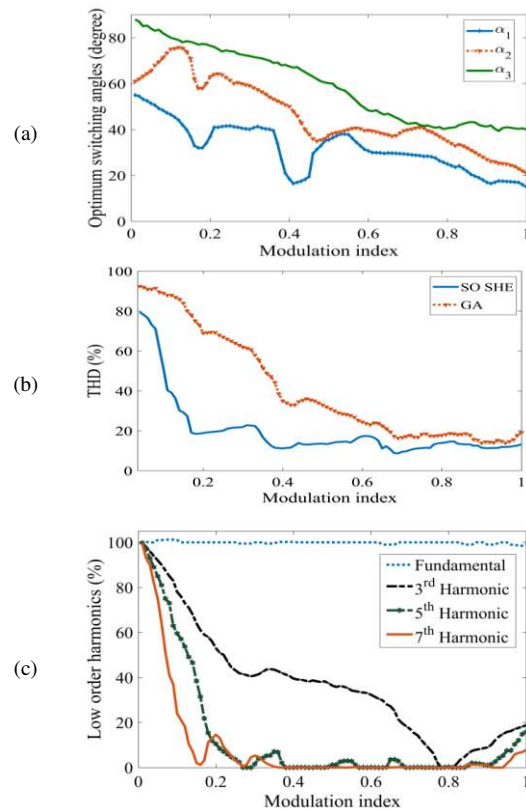
Fig. 6. (a) Switching angles obtained using SO SHE, (b) Comparison of THD (%) against M for GA and SO SHE, (c) Low order harmonics profile against M .
