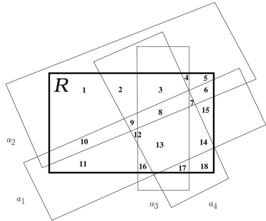
Fig. 2. Subregions generated in \mathcal{R} by intersection of acquisitions with each other and with region of interest. In this simple example, 18 subregions are generated.
