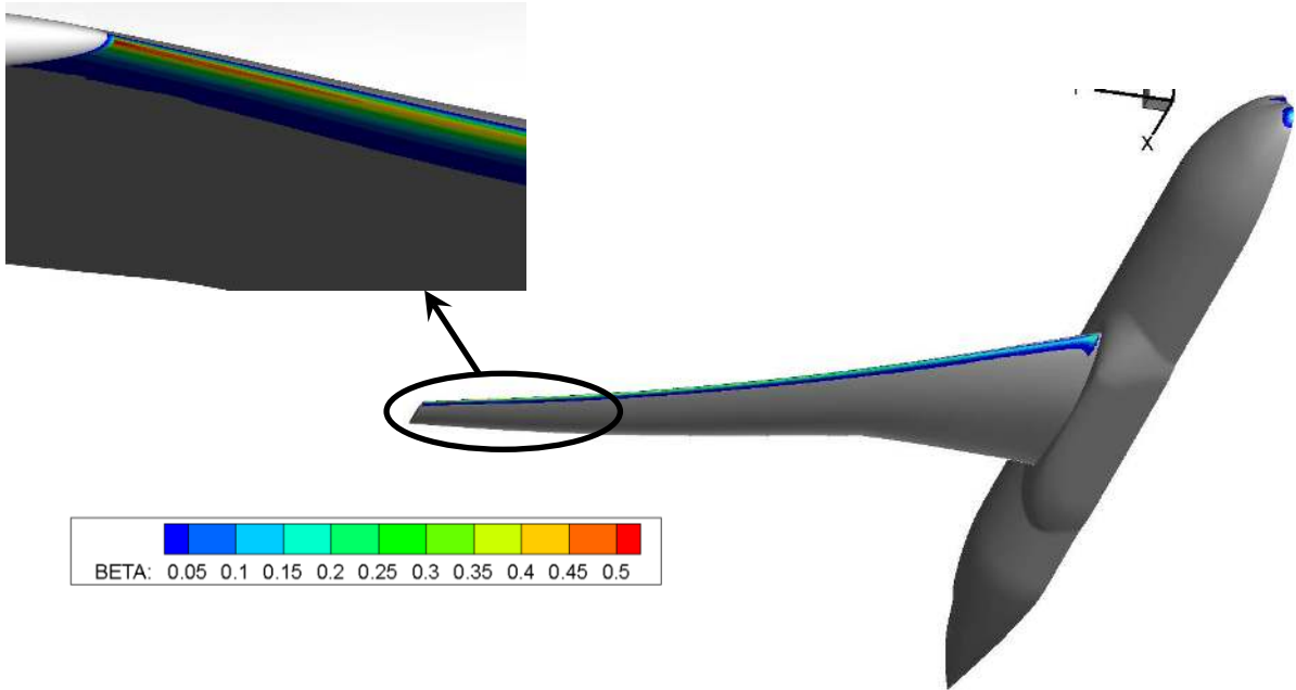
Figure 11. LEWICE3D local collection efficiency results for CRM65, droplet MVD = 20 \mu\text{m} , V = 232 knots, altitude = 10,000 ft.
