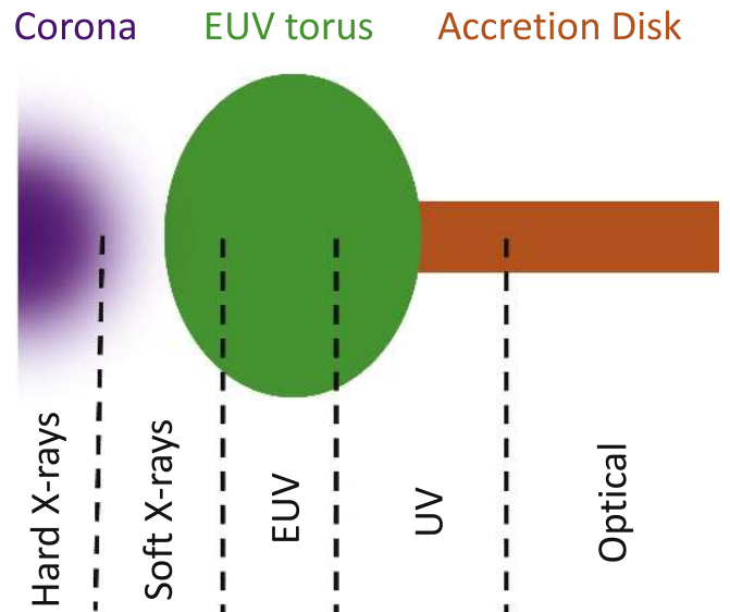
Figure 6. Sketch (not to scale) of the proposed geometry of the corona/EUV torus/accretion disk region, adapted from Gardner & Done (2017). The key difference between this and the standard lamp-post reprocessing model is the addition of the EUV toroidal-shaped component, which prevents the X-ray corona from directly illuminating the accretion disk. Instead, the corona illuminates and heats the proposed EUV component, which then thermalizes and illuminates the disk.
