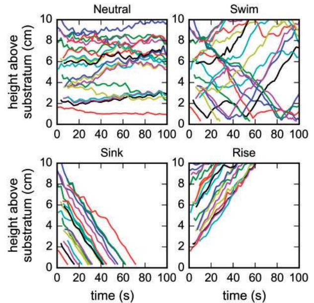
Fig. 5 Vertical positions of simulated larvae plotted as a function of time. A few larvae at the start of a video were chosen to represent different heights above the substratum, and their vertical positions at each time step are shown if they were passive and neutrally-buoyant (Neutral), actively swimming (Swim), passively sinking (Sink), or passively rising (Rise). The starting time in the wave cycle and the initial orientations and positions of the larvae in the water column were the same for all four plots. (This figure is available in black and white in print and in color at Integrative and Comparative Biology online.)
