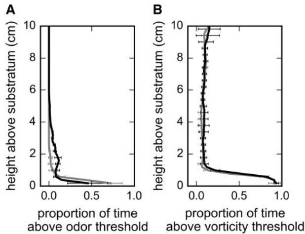
Fig. 4 Proportion of the time in a video lasting 31 s (approximately three wave cycles) that the odor concentration in the water was above \geq 0.1 B_{\text{mean}} ( A ), and that the vorticity was \geq 0.4 \text{ s}^{-1} ( B ) at different heights in the water column above a fouling community. Each curve represents a different fouling community. The mean values of all the points at a given height are plotted, and error bars show one standard deviation ( n = 980 pixels per height for odors; n = 60 grid points for vorticity).
