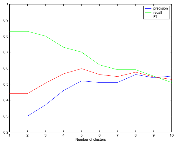
Figure 6: Average precision, recall and F1 measure for 2 to 10 clusters.
