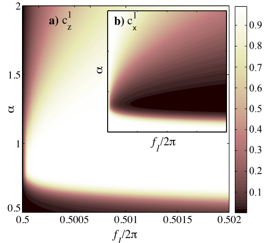
FIG. 2: For the Fig. 1b setup, coupling strengths as a function of the external flux f_1 and the qubit junction size \alpha = E_{J2}/E_{J1} , for f_2 = \pi/2 . We plot (a) the normalized first order coupling along the Z direction, c_z^1 \sigma_z \Delta\psi , and (b) across the XY plane.
