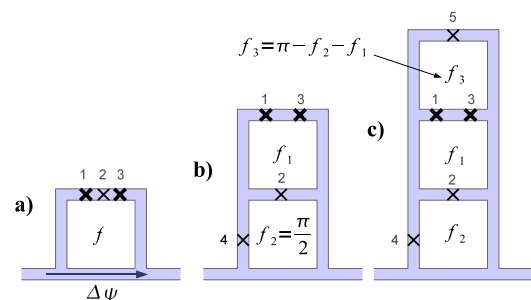
FIG. 1: Schemes for ultrastrong coupling between a qubit and a transmission line. (a) Basic setup of a qubit coupled directly to the line. \Delta\psi is the phase difference between the nodes in which the qubit and line intersect. (b) With a second loop, the coupling can be modulated. (c) A slightly improved setup in which the qubit is better decoupled from the flux f_2 .
