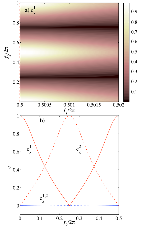
FIG. 3: (a) Following Eq. (5), normalized transverse coupling, c_x^1 , as a function of external fluxes f_1 and f_2 for the setup in Fig. 1c, using \alpha = 2.0 and \alpha_4 = 0.1 . (b) Cut at f_1 = 0.5 shows first-order (solid) and second-order couplings (dashed) of longitudinal ( c_z , blue) and transverse ( c_x red).
