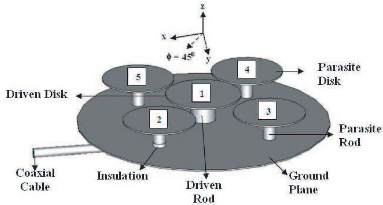
Figure 1. Disk-loaded monopole array antenna (No. 1 = driven element, No. 2–No. 5 = parasitic elements).
