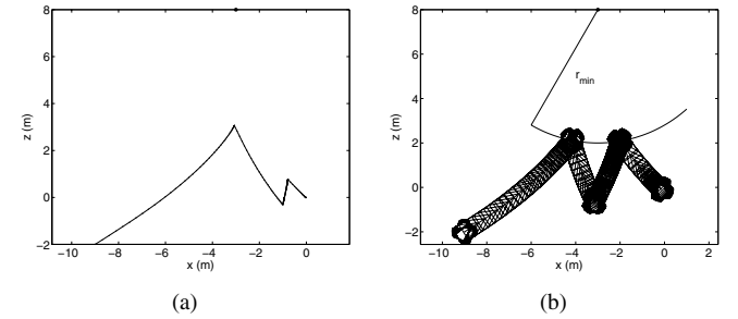
Fig. 9. (a) Simulation of two iterations with odometry drift of 0.8 deg/m. Pose after each iteration: (-1.00, -0.31, -2.63^\circ) and (-0.02, -0.01, -0.05^\circ) . (b) Simulation with minimum range constraint r_{min} = 6 m. Final pose (-0.15, -0.08, -0.40^\circ) .
