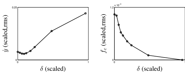
Figure 12. Root-mean-square (rms) values of the payload velocity and control force in z -direction under variation of \delta .
