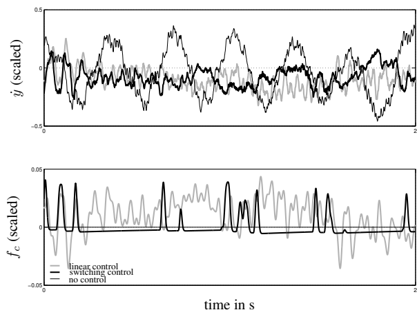
Figure 10. Time-series measurement of the payload velocity and control force in z -direction in case of no control, linear control, and switching control.
