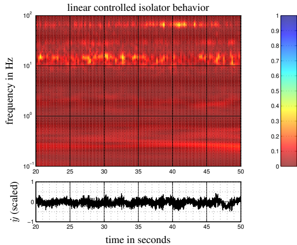
Figure 5. Time-frequency analysis of the measured and linear controlled z -velocity.
