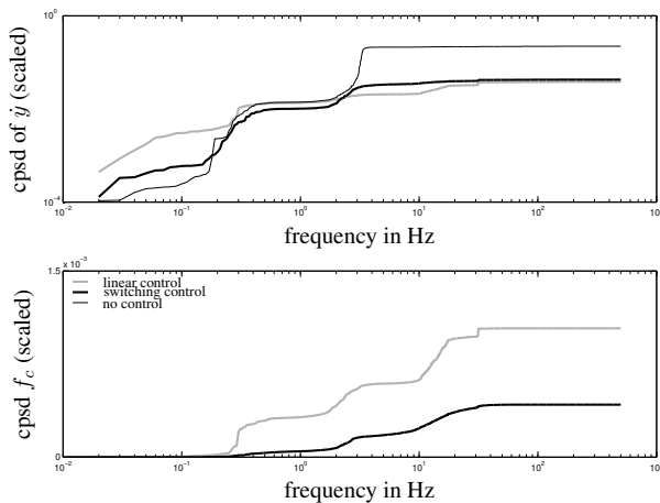
Figure 11. Cumulative power spectral density (cpsd) analysis of the payload velocity and control force in z -direction in case of no control, linear control, and switching control.
