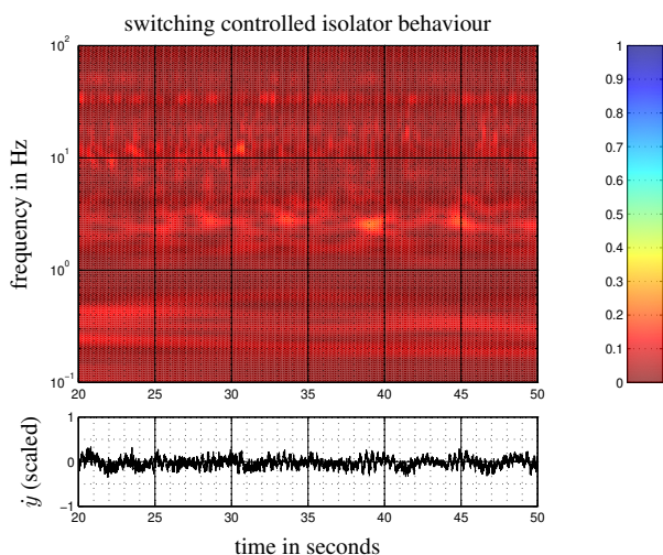
Figure 8. Time-frequency analysis of the measured and switching controlled z -velocity.
