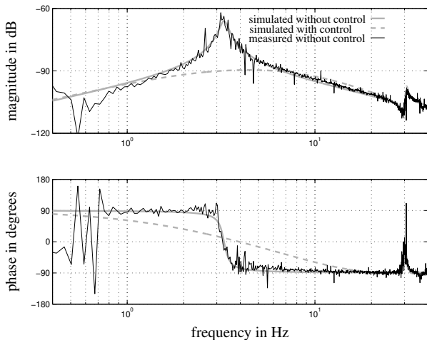
Figure 4. Bode representation of the isolator characteristics \mathcal{O}_l with ( \phi = 1 ) or without ( \phi = 0 ) control.
