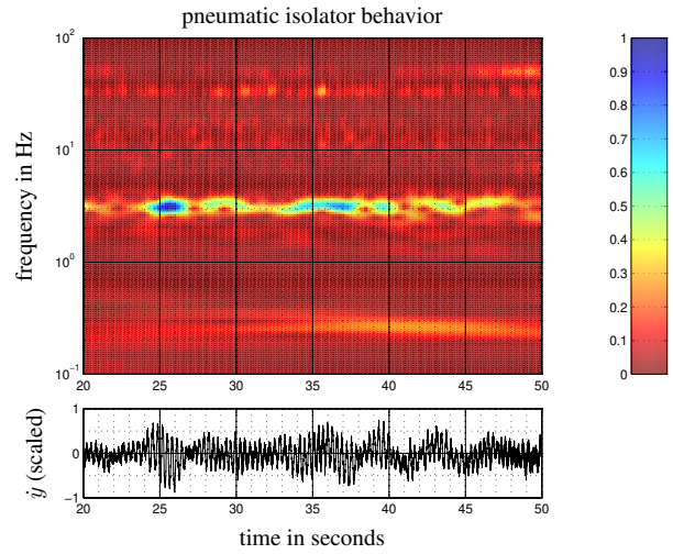
Figure 2. Time-frequency analysis of the measured z -velocity without active damping.
