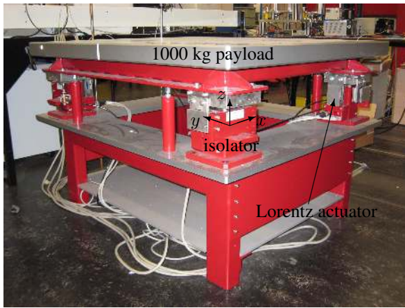
Figure 1. Vibration isolation system.
