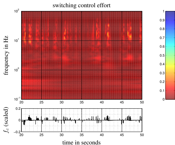
Figure 9. Time-frequency analysis of the measured switching control force.
