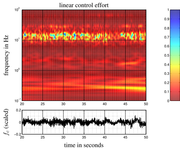
Figure 6. Time-frequency analysis of the measured control force in z -direction.
