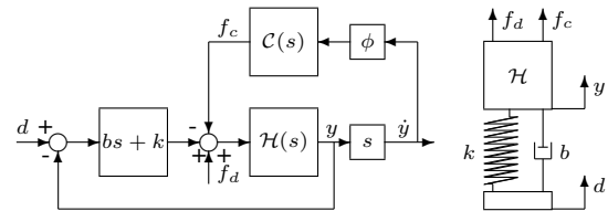
Figure 3. Simplified schematic of a controlled vibration isolator along with a mechanical representation.
