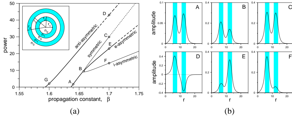
Fig. 1. (a) Power diagram of the ring nonlinear coupler. Dashed lines represent the unstable collapsing solutions. Inset: Sketch of the concentric ring coupler. Values used (in normalized units) are: r_1 = 5 , r_2 = 8 , r_3 = 11 and r_4 = 14 for radii and n_0 = 1 , n_1 = 2 for indices. (b) Examples of nonlinear stationary states corresponding to the points marked on the power diagram (labels A to F are correspondent in both subfigures).
