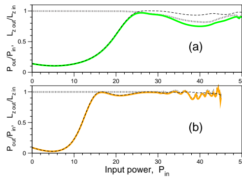
Fig. 4. Switching curves for the power (dark dashed lines) and angular momentum (light continuous lines) for (a) outer-waveguide excitation, and (b) inner-waveguide excitation. Also shown is the total angular momentum (dotted line).
