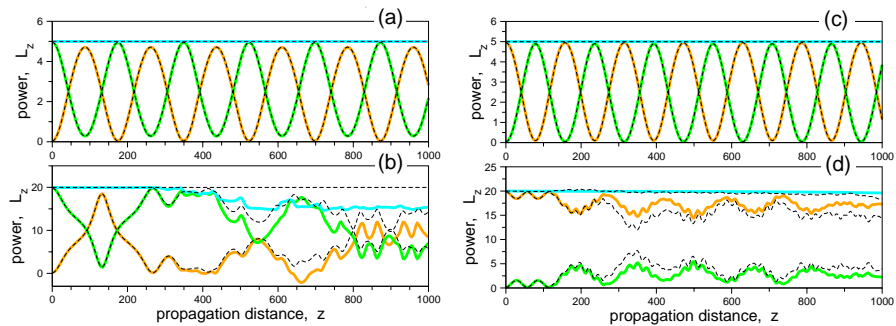
Fig. 3. Normalized power (dashed) and angular momentum (solid) vs. propagation distance for ring excitation with a single- charged vortex. The individual values for each core are plotted, together with the total values. (a) simulation for external-core excitation at P=5 ; (b) the same at P=20 ; (c) simulation for internal-core excitation at P=5 ; (d) the same at P=20 .
