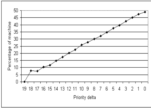
Figure 1: Long-term effect of multilevel queues with feedback mechanism on 2 jobs of differing priority. The X axis is the difference between the priorities of the 2 jobs. The net result over time is ‘proportional sharing’.
