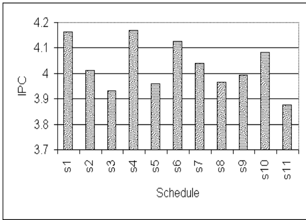
Figure 2: IPC of 8 jobs coscheduled 4 at a time, depending upon the sets chosen for coscheduling.
