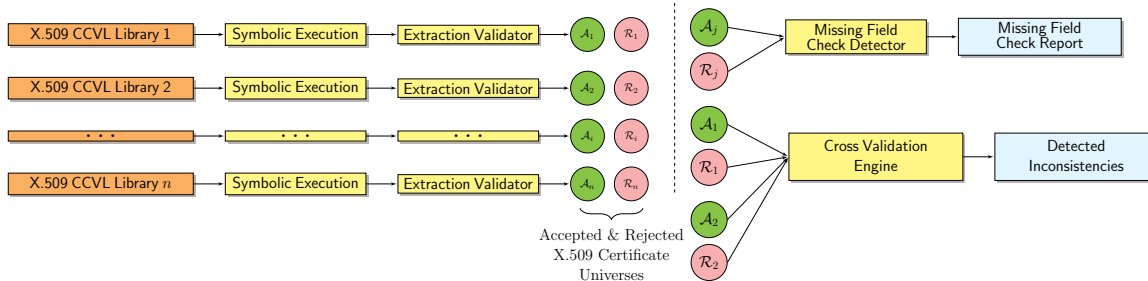
Fig. 1. Our noncompliance finding approach for X.509 CCVL implementations. Symbolic execution engine takes as input a CCVL implementation and extracts the approximated accepted and rejecting certificate universe whereas extraction validator validates it through concrete execution. Missing field check detector finds unscrutinized certificate fields from the universes. Cross validation engine performs cross validation among two implementations universes.
