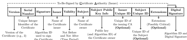
Fig. 2. A simplified structural view of an X.509 version 3 certificate (inspired by a similar figure in [89]).
