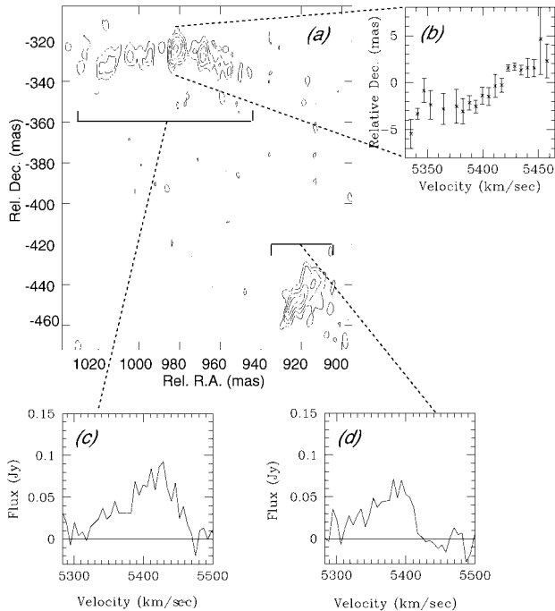
FIG. 2.—The eastern nucleus of Arp 220. (a) Image of the eastern nucleus of Arp 220 in the 1667 MHz OH line. The angular resolution and contour levels are the same as those in Fig. 1a, and the emission has been averaged over the velocity range 5300–5500 km s -1 . (b) Transverse velocity gradient across the bright central feature of component E1. Panels (c) and (d) show the integrated 1667 MHz spectra of components E1 and E2, respectively.
