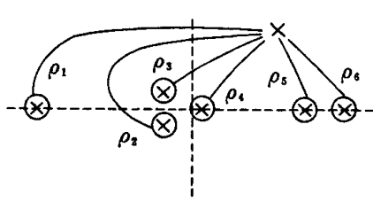
Figure (5.WI) ( \sqrt{g}=1+\varepsilon )
