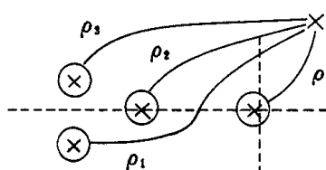
Figure (4.L) ( u=1+\epsilon )
