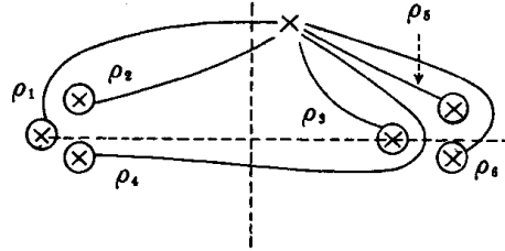
Figure (5.WII) ( \sqrt{g}=\varepsilon )
