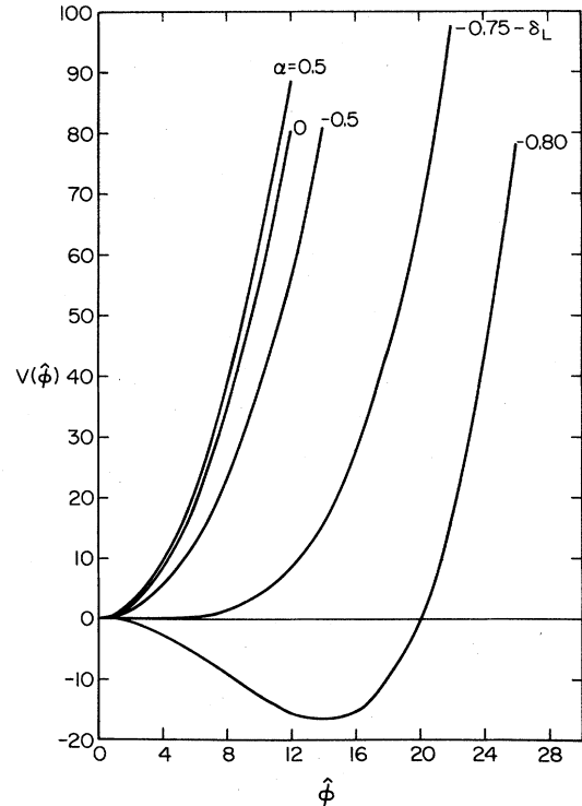
FIG. 1. One-loop effective potential of a massless, conformally coupled scalar field in a static Taub universe with varying deformation parameters ( \alpha ). The value \alpha=0 is the Einstein universe. Symmetry breaking will occur when \alpha < -0.75 - \delta_L , \delta_L = 6.302 \times 10^{-6}\lambda . Here we set a=1 , \lambda=10^{-2} , \hbar=1 . For all values of \hat{\phi}_0 such that |\hat{\phi}_0\alpha| < 4.2 \times 10^3 the quantum correction to the \phi^4 term is negligibly small compared to the classical term \lambda\phi^4/4! .
