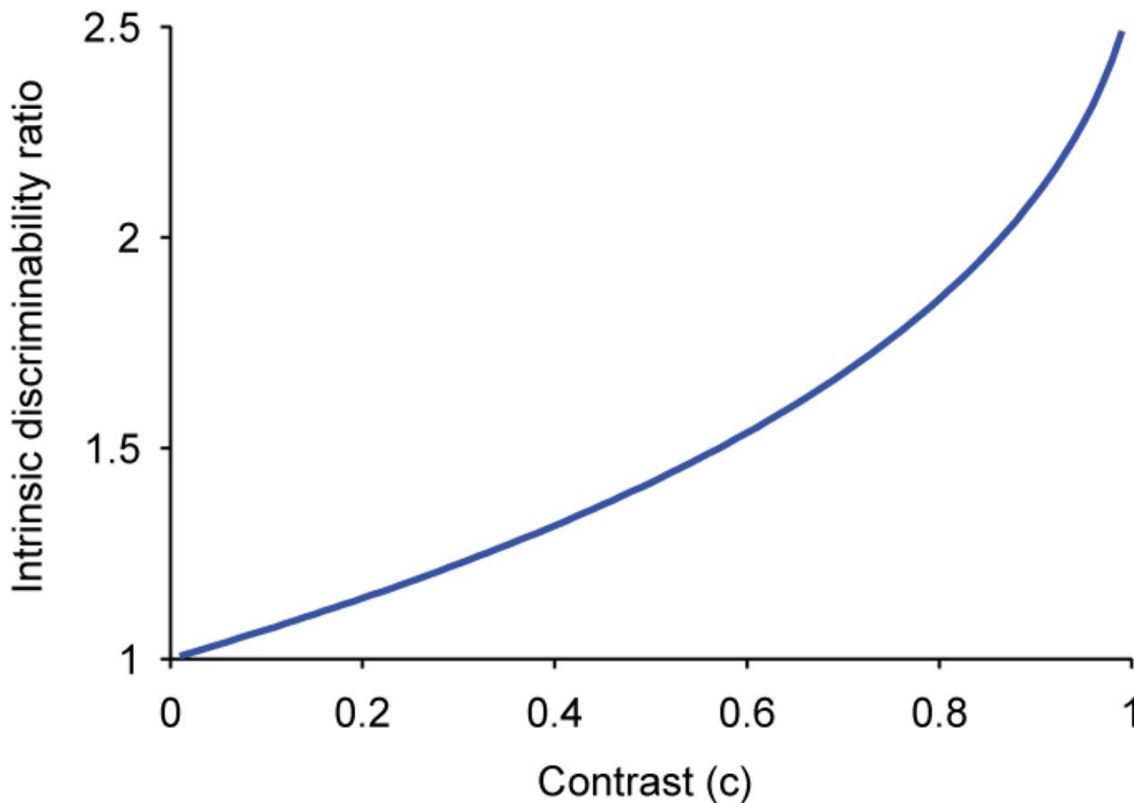
Fig. A. Decrements can be detected more readily than increments, and the asymmetry is an accelerating function of contrast
