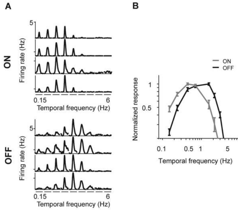
Fig. 2. Frequency tuning of ON and OFF cells diverges under scotopic conditions (A) Representative responses of four ON and four OFF ganglion cells to drifting sine wave gratings of increasing temporal frequency. (B) Average tuning curves (mean \pm SEM) for all ON and OFF cells, normalized to the peak ( n=20 ON cells, 31 OFF cells). On average the ON cells shifted to low frequencies, while the OFF cells continued to respond to high frequencies ( p < 10^{-3} , Student's t -test comparing the mean center of mass of the two populations). Note that under scotopic conditions, both ON and OFF cells fail to respond to the extreme high frequencies.
