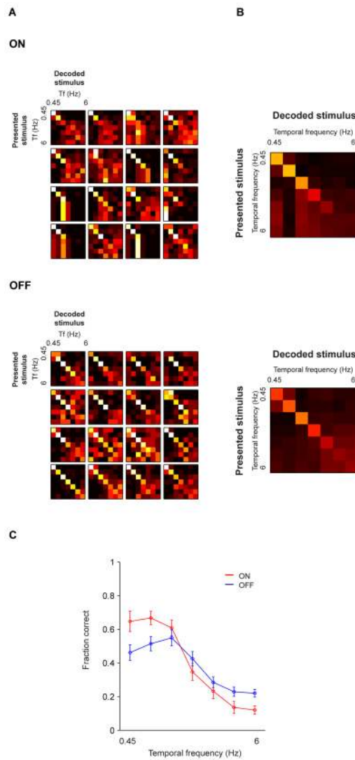
Fig. 6. Under scotopic conditions, there is a divergence in performance – ON cells perform better at low frequencies, while OFF cells perform better at high
