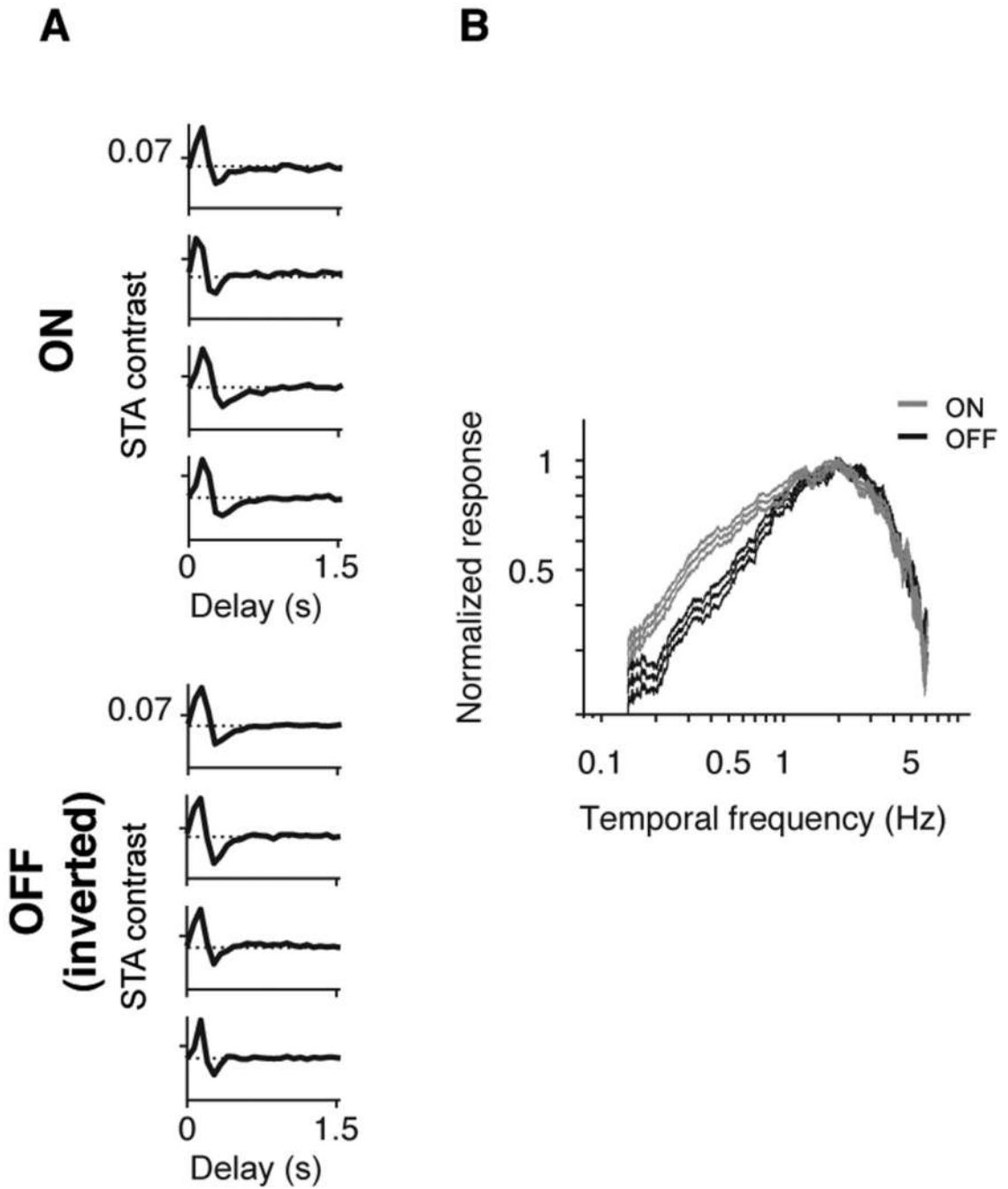
Fig. 3. ON and OFF cells show similar temporal response properties to white noise under photopic conditions
