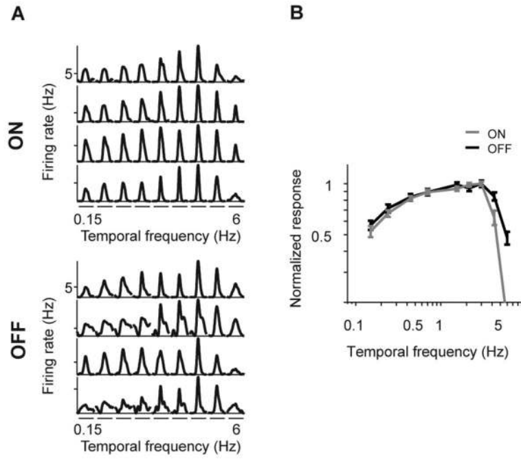
Fig. 1. ON and OFF cells show similar temporal frequency tuning in response to sine wave gratings under photopic conditions
