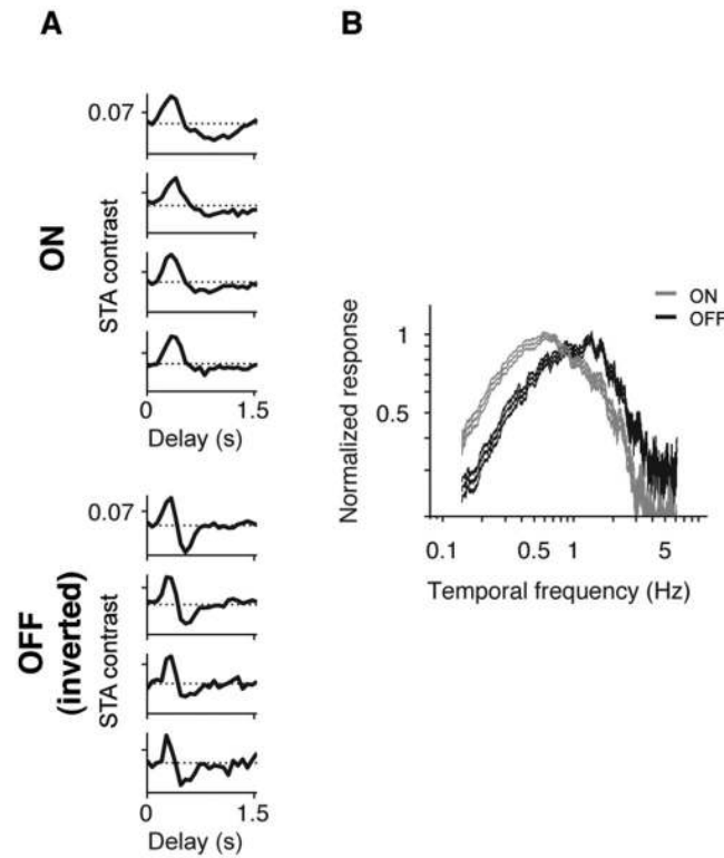
Fig. 4. The divergence under scotopic conditions was also observed for the white noise stimulus (A) Representative STA time courses for four ON and four OFF ganglion cells in response to a white noise (random checkerboard) stimulus. (B) Average temporal frequency responses (mean \pm SEM), normalized to the peak ( n=20 ON cells, n=31 OFF cells). As with the grating stimulus, the ON cells shifted to low frequencies, while the OFF cells continued to respond to high frequencies ( p < 10^{-3} , Student's t -test comparing the mean center of mass the two populations).
