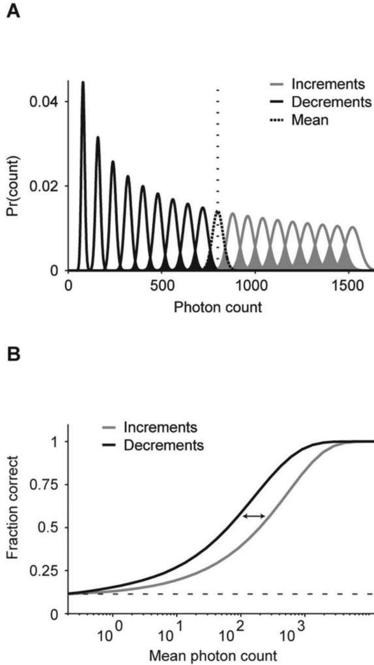
Fig. 7. At low light levels, increments become harder to discriminate than decrements of equal magnitude, due to asymmetries in the Poisson distribution
