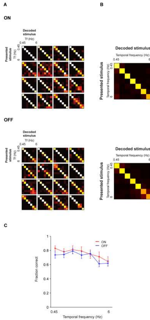
Fig. 5. Under photopic conditions, it is possible to decode across the entire range of temporal frequencies using responses of ON or OFF cells
