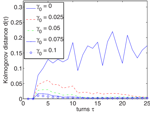
FIG. 2. (Color online) Kolmogorov distance d(\tau) against the number of turns ( \tau ) of the cyclic QWs in the noiseless and noisy cases with n=51 . For the unitary case ( \lambda=0 ; bold line) the walk becomes increasingly asymmetric as the number of turns is increased, until about 7–10 turns, after which it fluctuates around d \approx 0.15 . The plots represent generalized amplitude damping noise at different noise levels at temperature T=3.5 (in units where \hbar \equiv k_B \equiv 1 ), \Delta=0.1 , and \theta=30^\circ . The walker is evolved with the initial state parameters (in degrees) \theta_0=30^\circ , \varphi_0=40^\circ , with B(20^\circ, 10^\circ, 30^\circ) and G(40^\circ, 50^\circ) .
