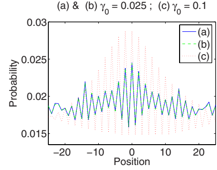
FIG. 3. (Color online) Position probability distribution for a Hadamard walk B(0, 45^\circ, 0) on an n cycle ( n=51 ) with initial state (1/\sqrt{2})(|0\rangle + |1\rangle) when subjected to generalized amplitude damping noise with \Delta=0.1 and finite T (=6.0) for \tau=11 . (a), (b) \gamma_0=0.025 , (b) is the distribution for the QWs augmented by operation G(30^\circ, 50^\circ) ; note the walk remains quantum yet with symmetry almost completely restored; (c) classicalized pattern (indicated by the regular envelope) obtained with larger noise level corresponding to \gamma_0=0.1 .
