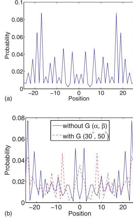
FIG. 1. (Color online) Position probability distribution for a Hadamard walk B(0^\circ, 45^\circ, 0^\circ) on (a) a line and (b) an n -cycle, with ( n=51 ) and initial state (1/\sqrt{2})(|0\rangle + |1\rangle) , for the unitary case ( \gamma_0=0 ). Each figure presents the distribution with and without being subjected to the phase operation G(30^\circ, 50^\circ) . In (a), there is perfect symmetry, since both distributions coincide. In (b) the two plots do not overlap, indicating the breakdown of the symmetry.
