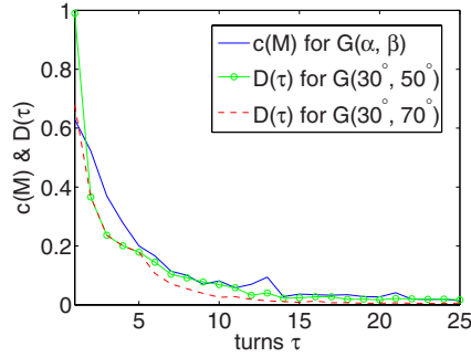
FIG. 4. (Color online) Normalized coherence function c(M) (bold) and the normalized Kolmogorov distance D(\tau) (dashed) for a cyclic QWs as a function of turns \tau . An overall reduction of both c(M) and D(\tau) with time is seen for the generalized amplitude damping noise characterized by temperature T=3.5 and \Delta=0.1 . The Hadamard walk is evolved with the initial state parameters (in degrees) \theta_0=45^\circ , \varphi_0=0^\circ , and G(\alpha, \beta) . The line-with-circle plot represents D(\tau) with G(30^\circ, 50^\circ) and dashed line represents G(30^\circ, 70^\circ) . The c(M) (solid line) remains roughly the same for both pairs of \alpha and \beta . For a clear depiction of the notion of symmetry restoration in the walk even in the quantum regime, cf. Fig. 3.
