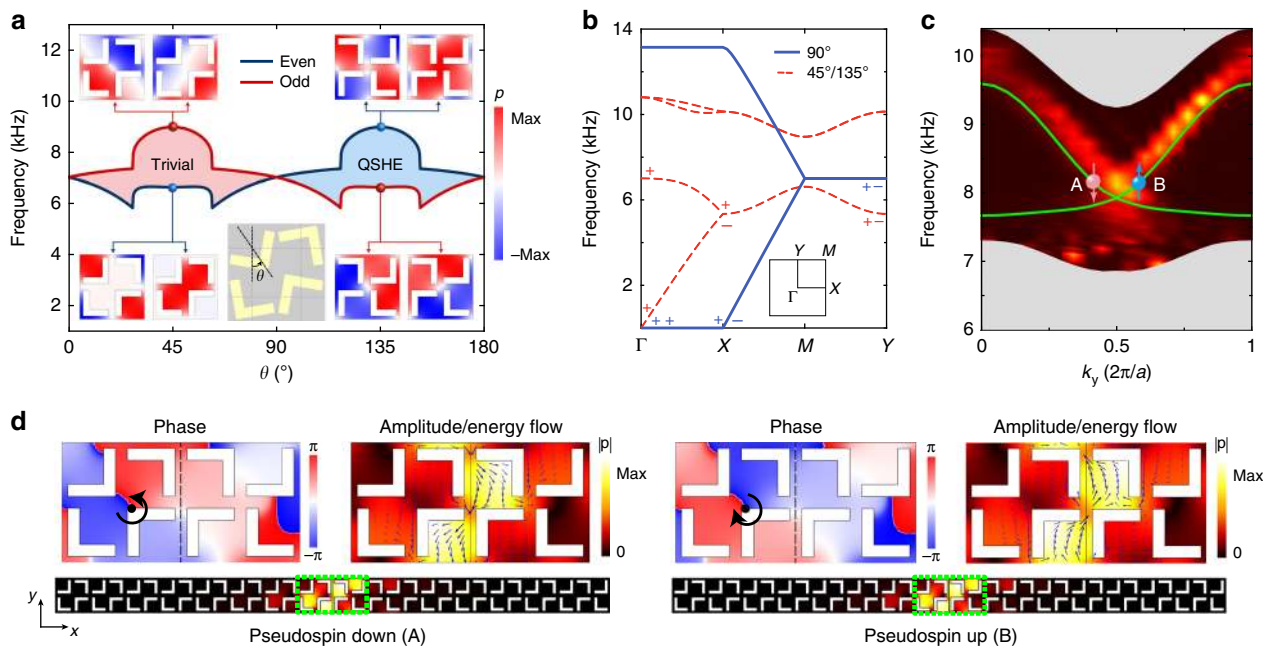
Fig. 5 Acoustic quantum spin Hall effect and helical edge states in the lowest band gap. a Evolution of the bulk bands and parities at the M point (including two doublets of even and odd parities) by tuning the rotation angle of the scatterers, \theta (defined in the inset). Acoustic pressure profiles of the doublets at the four marked points are shown as the insets. The parity inversion indicates that the blue region mimics the quantum spin Hall insulator in acoustic systems, while the red region corresponds to the trivial band gap. b Acoustic bands for \theta = 90^\circ, 45^\circ, and 135^\circ . The symbols +/- represent, respectively, the even/odd parity for the \Gamma, X, and Y points for the lowest two bands. c Measured (hot color) and calculated (green) dispersions of helical edge states in the lowest band gap at the boundary between two sonic crystals with different \theta 's, 45^\circ, and 135^\circ . The gray regions denote the bulk bands. d Acoustic pressure profiles for two edge states marked by the red and blue dots in c , with amplitude (hot color), Poynting vectors (blue arrows) and phase profiles shown near the boundary (the green-box regions at the bottom panel). Geometry parameters (except for the rotation angle \theta ) are the same as that in Fig. 1.
