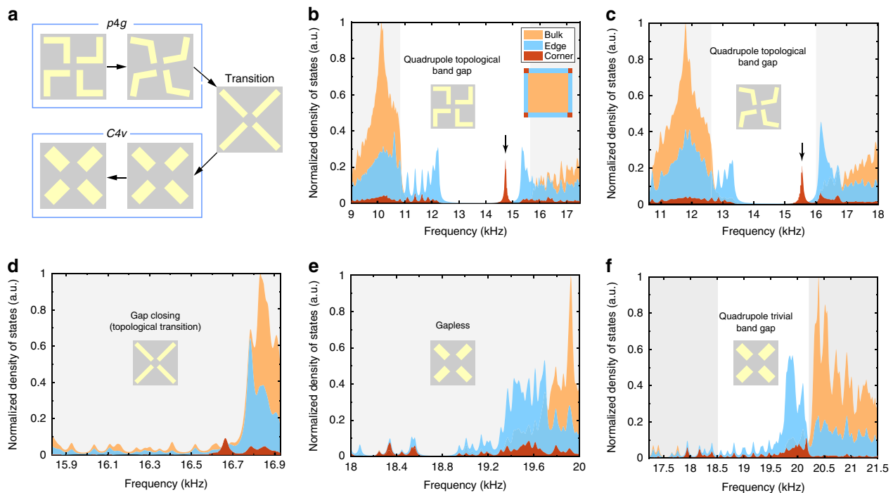
Fig. 2 Topological phase transitions in the second band gap. a Topological phase transitions induced by continuously tuning the geometry (indicated by the arrows): first decrease the arch height h to 0 (the first three structures), then reduce the length l (the fourth structure), and finally increase the width w (the fifth structure). The corresponding geometric parameters are h = 0.21a , l = 0.42a , w = 0.1a for the first structure; h = 0.15a , l = 0.42a , w = 0.1a for the second structure; h = 0 , l = 0.42a , w = 0.1a for the third structure; h = 0 , l = 0.25a , w = 0.18a for the fourth structure; and h = 0 , l = 0.25a , w = 0.21a for the fifth structure. The first two structures have p4g symmetry, whereas the others have C_{4v} symmetry. b–f Calculated local density-of-states for the corner, edge, and bulk regions. The densities-of-states are normalized so that the peak values in the figures are 1. Here, a.u. stands for arbitrary units. The corner, edge, and bulk regions are sketched in the inset of b . The calculations are performed on a box-shaped finite structure consisting of 10 \times 10 sonic crystal unit cells enclosed by hard-wall boundaries. An air channel of width 0.25a separates the sonic crystal and the hard-wall boundaries to ensure the physical edges and corners for the acoustic waves.
