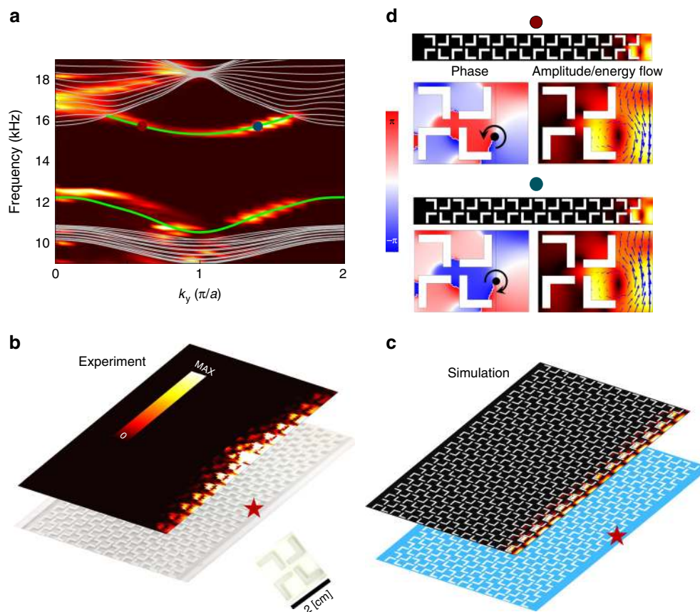
Fig. 3 Gapped topological edge states induced by anomalous quadrupole in the second band gap. a Measured (hot color) and calculated (green) dispersions of the acoustic edge states. Gray curves represent calculated acoustic bulk bands. b, c Top: measured and simulated acoustic pressure profiles of the edge states launched by a point-like source (indicated by the red stars), respectively. Below: photo of the fabricated sample and the illustration of the structure, respectively. Inset in b : photo of a unit-cell. d Acoustic pressure profiles for the two edge states marked by the red and blue dots in a , with phase, amplitude and Poynting vectors (blue arrows) shown near the edge. Phase vortex centers and phase winding directions are marked by the black dots and arrows, respectively. The edge is formed between the sonic crystal and the hard-wall boundary made of photosensitive resin. Unit-cell geometry parameters are the same as that in Fig. 1.
