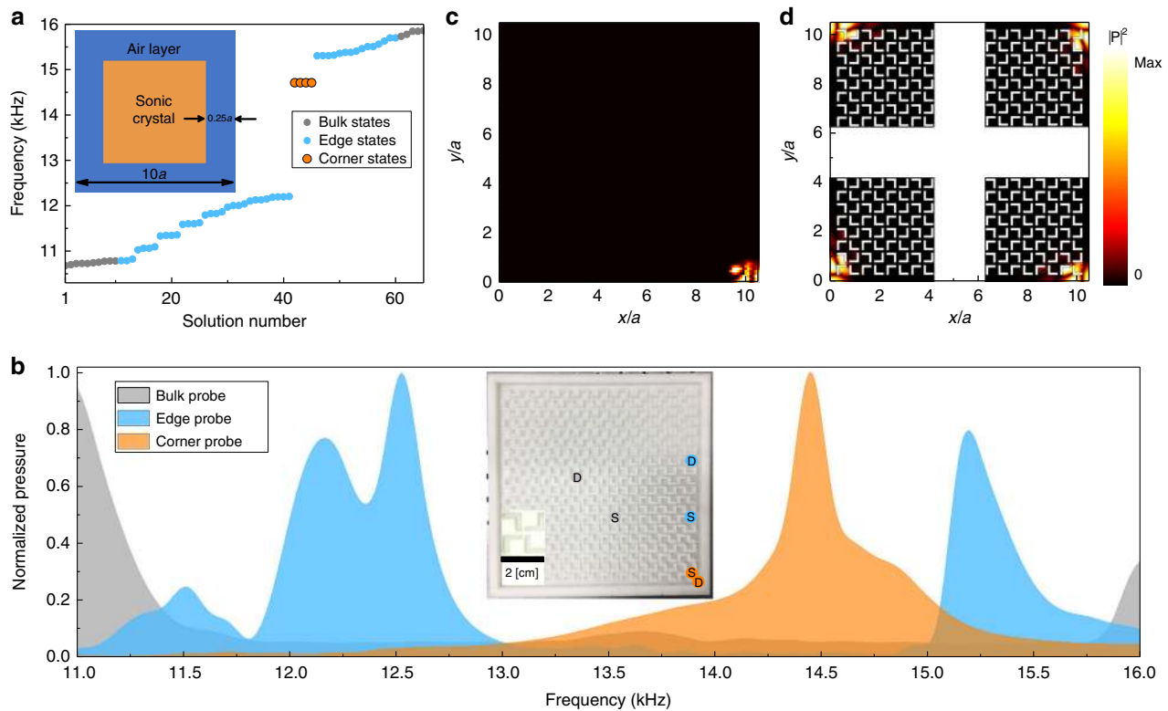
Fig. 4 Topological corner and edge states in the second band gap due to the anomalous quadrupole. a Calculated acoustic spectrum for a box-shaped finite structure consisting of 10 \times 10 sonic crystal unit cells enclosed by hard-wall boundaries with an air channel of width 0.25a separating them (see the inset for the structure illustration). b Frequency-resolved transmission spectra for three pump-probe configurations: bulk probe, edge probe and corner probe. Inset: photo of the sample with a zoom-in photo of the unit-cell. Source (“S”) and detector (“D”) for each pump-probe configuration (including the bulk, edge, and corner probes) are marked in the inset using the same color as that of the corresponding transmission curve. c, d Measured and simulated acoustic pressure profiles of the corner states, respectively. Four degenerate corner states (related by the C_4 rotation) are shown in d , whereas only one of them is measured in c . Unit-cell geometry parameters are the same as that in Fig. 1.
