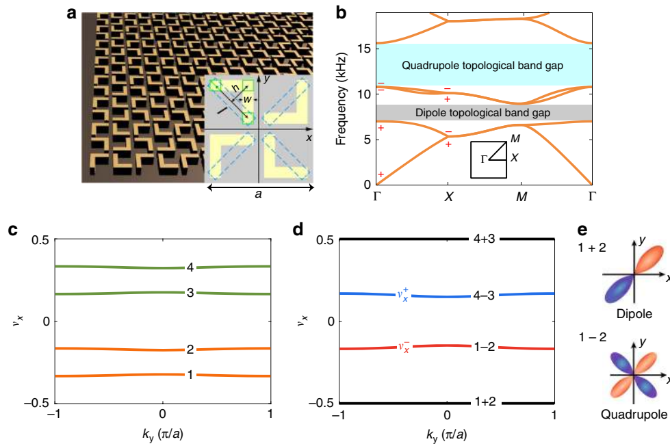
Fig. 1 Symmetry-protected hierarchy of anomalous topological multipoles in nonsymmorphic sonic crystals. a A bird’s-eye view of the 2D nonsymmorphic sonic crystal cladded by plastic boards from below and above (not shown). The inset illustrates the unit-cell structure with four arch-shaped scatterers made of photosensitive resin (an acoustically rigid material). b Acoustic bands and the hierarchy of multipole topological band gaps. The dipole and (anomalous) quadrupole are quantized and protected by the glide symmetries in the p4g group. Inset: Brillouin zone. Symbols +/- represent even/odd parity, respectively, at the \Gamma and X points in the Brillouin zone. c Gapped and nondegenerate Wannier bands for the anomalous quadrupole topological gap. d Wannier bands for the sum (“ 1 + 2 ” and “ 4 + 3 ”) and difference (“ 1 - 2 ” and “ 4 - 3 ”) sectors. e Schematic illustration of the linear combinations of the Wannier orbits in different sectors (“ 1 + 2 ” and “ 1 - 2 ”), which respectively yield the dipole topology and the anomalous quadrupole topology. Unit-cell geometry parameters are h = 0.21a , l = 0.42a , w = 0.1a , and a = 2 cm.
