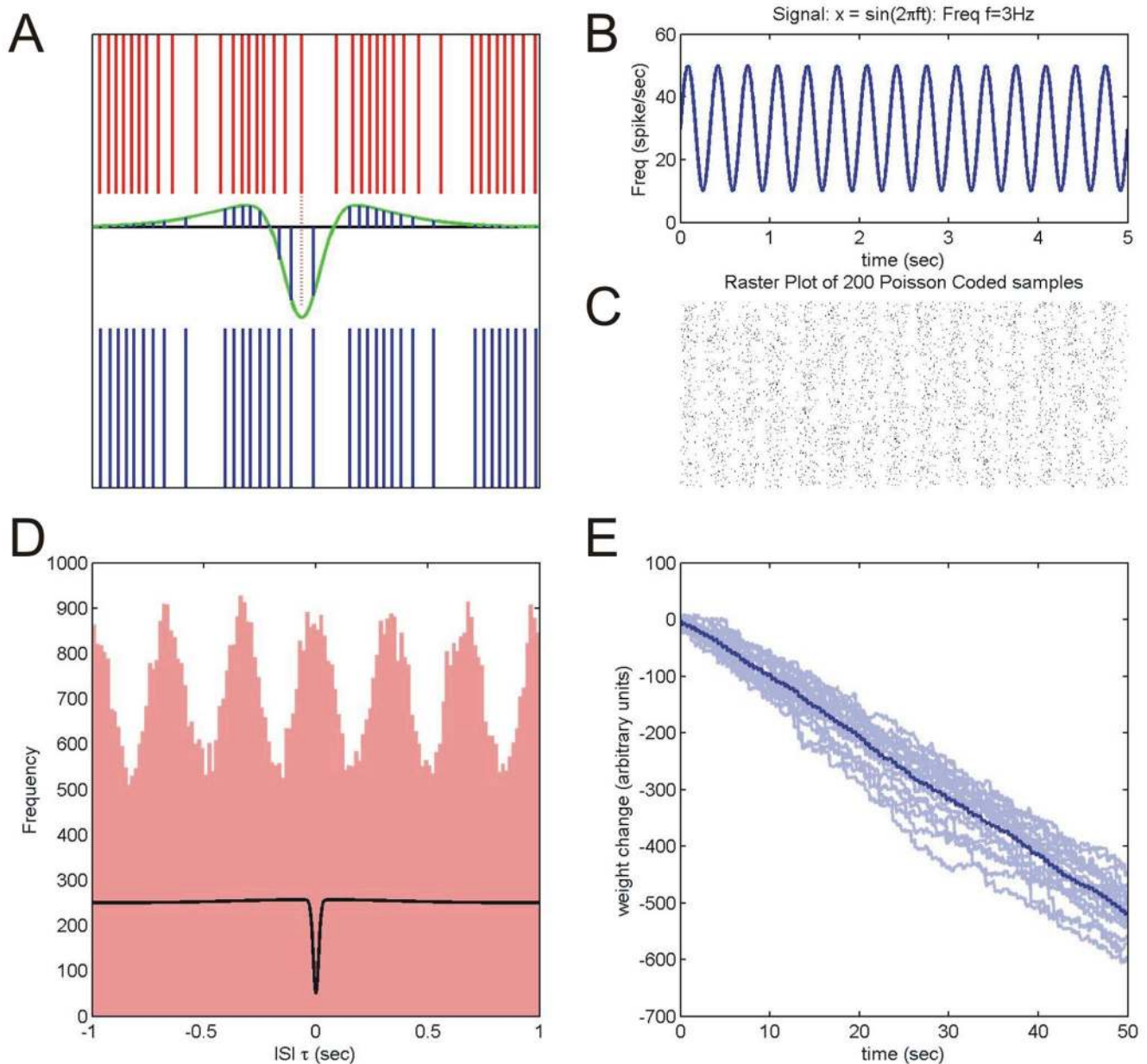
Figure 9. iSTDP for stochastic inputs. A: The top (red) spike train represents vestibular input x and the bottom (blue) spike train represents inhibitory cerebellar input y . The green curve shows an iSTDP profile (corresponding to a difference of Gaussians kernel -K(\tau) as described in Methods) chosen to demonstrate both LTP and LTD lobes clearly. The total contribution of a given vestibular spike, for example the one extended by the red dotted line, to synaptic weight change is calculated as follows: its timings \tau_{ij} with respect to all cerebellar spikes are determined. The contribution of each of these spike pairs to weight change is proportional to -K(\tau_{ij}) (equation (3)), these values are shown graphically as the blue segments under the iSTDP profile centered at the chosen vestibular spike. The sum of all these segments is the weight change 'caused' by that vestibular spike. B: A sinusoidal vestibular input modulating at 3 Hz, represented as a variation in firing rate with mean rate 30 Hz and amplitude 20 Hz. C: A raster plot of 200 different Poisson coded samples of the sinusoidal signal (for Poisson coding the probability of a spike in a short interval dt is Fdt where F is the firing rate to be coded). It is clear that the coding scheme is asynchronous, i.e. the timing of individual spikes is not well-determined. D: A histogram of all interspike intervals \tau (between vestibular and cerebellar spikes, see Methods) for a single 50 s x,y input pair modulated in phase at 3 Hz and Poisson coded as in Fig. 2. Despite the fact that individual spikes are not precisely timed, there is a clear modulation of the ISI histogram at 3 Hz with a peak at zero ISI. The experimentally constrained iSTDP profile from Fig. 3H is overlaid on the histogram. E: Cumulative weight change calculated for 20 pairs of 50 s samples of vestibular and cerebellar input. There is a stochastic but consistent weight decrease. The mean weight change (dark blue curve) is also shown. doi:10.1371/journal.pone.0013182.g009
