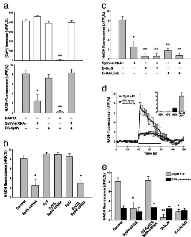
Fig. 5. Syt IV is necessary for Ca^{2+} -dependent glutamate release from astrocytes. (a) Expression of SS-Syt IV does not affect glutamate release or Ca^{2+} signaling induced by ATP (20 \mu M), but leads to a recovery of release when expressed in the presence of Syt IV-siRNA. Because the changes in glutamate release are independent of the amplitude of the Ca^{2+} signal, they support the notion that Syt IV is required downstream of the Ca^{2+} signal to control transmitter release (*, P < 0.05 ; **, P < 0.01 ). Data were collected from 18 (calcium imaging) and 12 (glutamate assays) trials obtained from two independent sets of cultures. (b) Syt I but not Syt V can rescue glutamate release after Syt IV-siRNA treatment ( P < 0.01 ). (c) Mutations of amino acids homologous to Syt I C2B domain amino acids that coordinate Ca^{2+} binding (B-D 1,2 N and B-D 3 N,E 4 Q) lead to dominant-negative effects on astrocytic glutamate release (*, P < 0.05 ; **, P < 0.01 ). All modifications to release (except N,N,N',N'-tetraacetate) are independent of changes in ATP-evoked Ca^{2+} mobilization. (d) Hypoosmotic saline induces the release of glutamate from astrocytes (black circles), which is comparable with ATP-evoked glutamate release (gray circles). The black horizontal bar represents the application of stimuli (ATP or hypoosmotic saline). (e) Syt IV-siRNA and Syt IV dominant-negative mutations significantly depress ATP-induced, Ca^{2+} -dependent glutamate release (gray bar, *, P < 0.05 ; **, P < 0.01 ) but have no effect on hypoosmotic saline-induced glutamate release (black bar). Data shown in b–e were collected from 12 trials obtained from two independent cultures.
