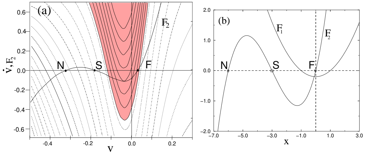
FIG. 2. (a) Function plot of F_2(v) and contour plot of F_1(v, \dot{v}) for the Morris-Lecar model. The dark area corresponds to the negative dissipation, i. e. , F_1 < 0 . (b) Function plots of F_1(x) and F_2(x) for the MVP model.
