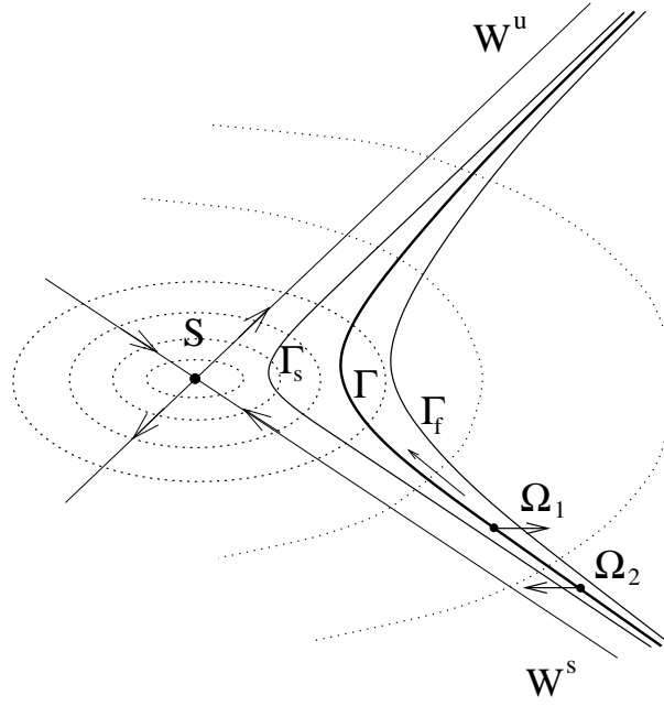
FIG. 4. Phase flows near the saddle ( S ).
