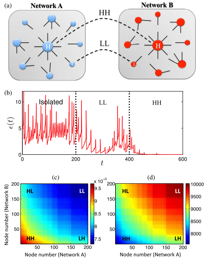
FIG. 1 (color online). (a) Schematic representation of the interconnection of two heterogeneous networks. HH corresponds to a strategy connecting high-degree nodes and LL to the connection between low-degree nodes. (b) Synchronization error \epsilon(t) of two interconnected Barabási-Albert networks of N = 200 Rössler oscillators at three different stages: isolated, interconnected following a LL strategy, and replacing the LL connection with a HH one. Equations of the Rössler system are given in [27] and the parameters used in the simulations are a = b = 0.2 and c = 5.7 . \epsilon(t) is obtained as the average across all pairs of oscillators of the pairwise distance in three dimensional phase space, 2/N(N-1) \sum_{i < j} \|\mathbf{x}_i - \mathbf{x}_j\| , where \mathbf{x}_i is the state vector of oscillator i and \|\cdot\| denotes the (Euclidean) norm. (c) \lambda_2 of the NON obtained from connecting two N = 200 Barabási-Albert networks with one interlink, in all possible configurations. The node numbers are ordered according to the node degree and, when coinciding, the eigenvector centrality. (d) Eigenratio r = \lambda_N/\lambda_2 for the same case as (c).
