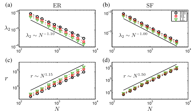
FIG. 3 (color online). Dependence of synchronizability of class II and III systems on the size of the networks N . Averaged second eigenvalue \lambda_2 [(a) and (b)] and r [(c) and (d)] over 30 realizations of two Erdős-Rényi networks and two scale-free networks of average degree \bar{k} = 12 . See Section S2 of [29] for details.
