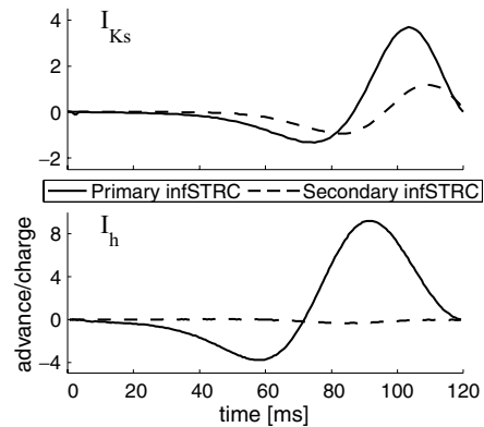
Figure 10. Demonstration of secondary infSTRC. The infSTRC (see Eq. (3)) shows the neuron's response to weak, brief pulses of injected current. For primary infSTRCs (solid lines), advances are measured in the same cycle that the pulse is injected. Secondary infSTRCs (dashed lines) show any residual perturbations in spike timing during the following cycle. In the case of I_h (bottom panel), the secondary infSTRC is essentially zero as the neuron returns to its natural period in the cycle after the perturbation. In the case of I_{Ks} (top panel), the effect of the pulse persists into the second cycle.
