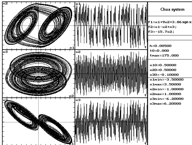
Fig. 5. A chaotic trajectory of the switch Chua circuit (8) obtained with the explicit Euler method. (a) Phase portraits and
