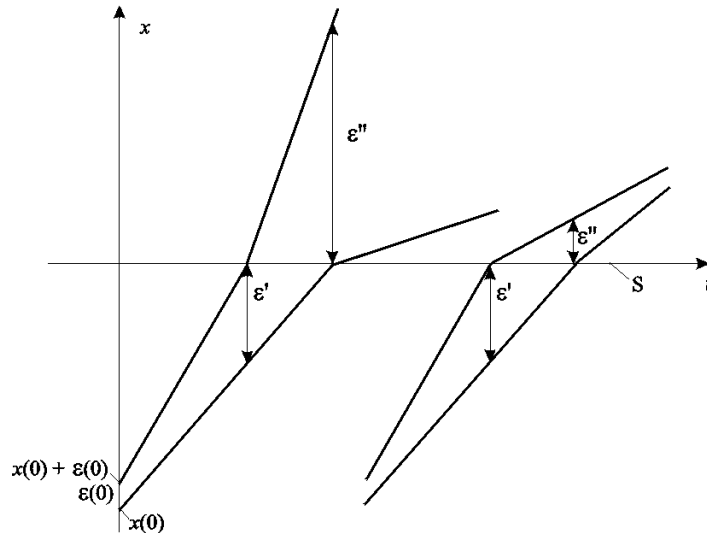
Fig. 9. The divergence of two closed trajectories in the phase space [0, \infty) \times R near the discontinuity surface S, x = 0 . (a) The distance between the trajectories still increases after the surface crossing: the system behavior could remain chaotic; (b) The distance decreases, and the motion could be not chaotic after the crossing (schematically).
