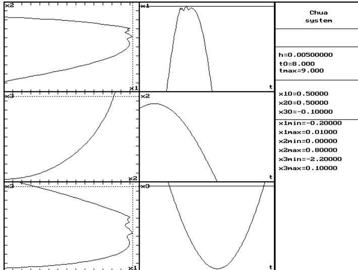
Fig. 7. Detail of a chaotic trajectory. Due to x_1 discontinuity, only this component presents corners near the discontinuity surface x_1 = 0 .
