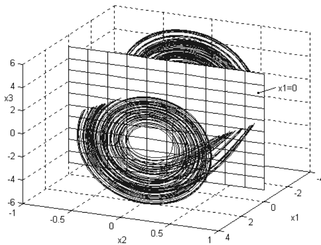
Fig. 6. Three-dimensional view of a chaotic trajectory and
