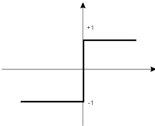
Fig. 2. The graph of the set-valued function Sgn(x) .
