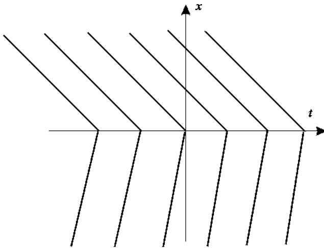
Fig. 1. Solutions of the equation \dot{x}=1 - 2sgn(x) , for x \neq 0 .
