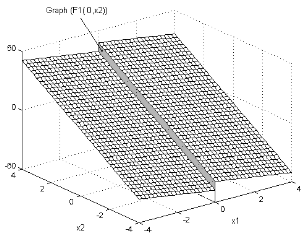
Fig. 3. (a) The graph of the first component, f_1 , of the right-hand side of (8); (b) The graph of the corresponding set-valued
