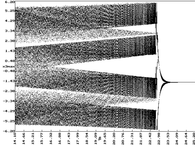
Fig. 4. Bifurcation diagram of the component x_3 max of the dynamical system (8) versus the control parameter \beta .
