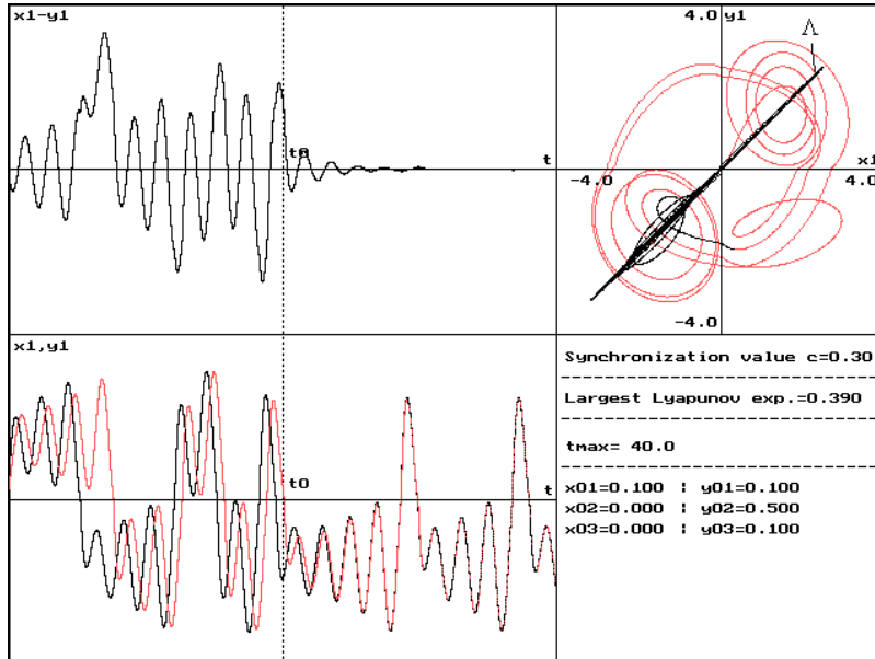
Fig. 10. Synchronization of two identical switch Chua circuits modeled by (8).
