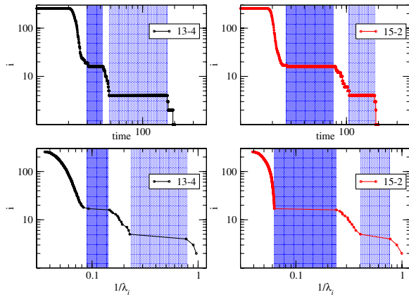
FIG. 2 (color online). Top: Number of disconnected synchronized components (equivalent to number of null eigenvalues of S[\mathcal{D}_T(t)] ) as a function of time for the two networks of Fig. 1 at T = 0.99 . Bottom: Rank index i (see text) versus the inverse of the corresponding eigenvalues of the Laplacian matrix \mathcal{L} . The shadow regions indicate the stability plateaus for 16 (dark) and 4 (light) communities. The same representation is used for the plateaus in the eigenvalue spectrum corresponding to indices 16 and 4.
