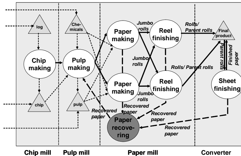
Figure 3 : Processes and material flows in an integrated pulp and paper mill
