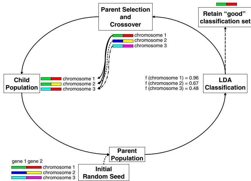
Figure 2. Genetic algorithm–linear discriminant analysis. An initial seed is used to create the first parent generation of chromosomes (possible sets) of genes ( z_{ij}^0 ). Chromosomes yielding good classifications are retained based on the classification results from the LDA (posterior probabilities). Each chromosome in the child generation is born from two parent chromosomes, which are probabilistically selected on the basis of their classification scores. Additionally, the best chromosome from each generation is carried over to the child generation (elitism). Finally, the child generation becomes the next parent generation.
