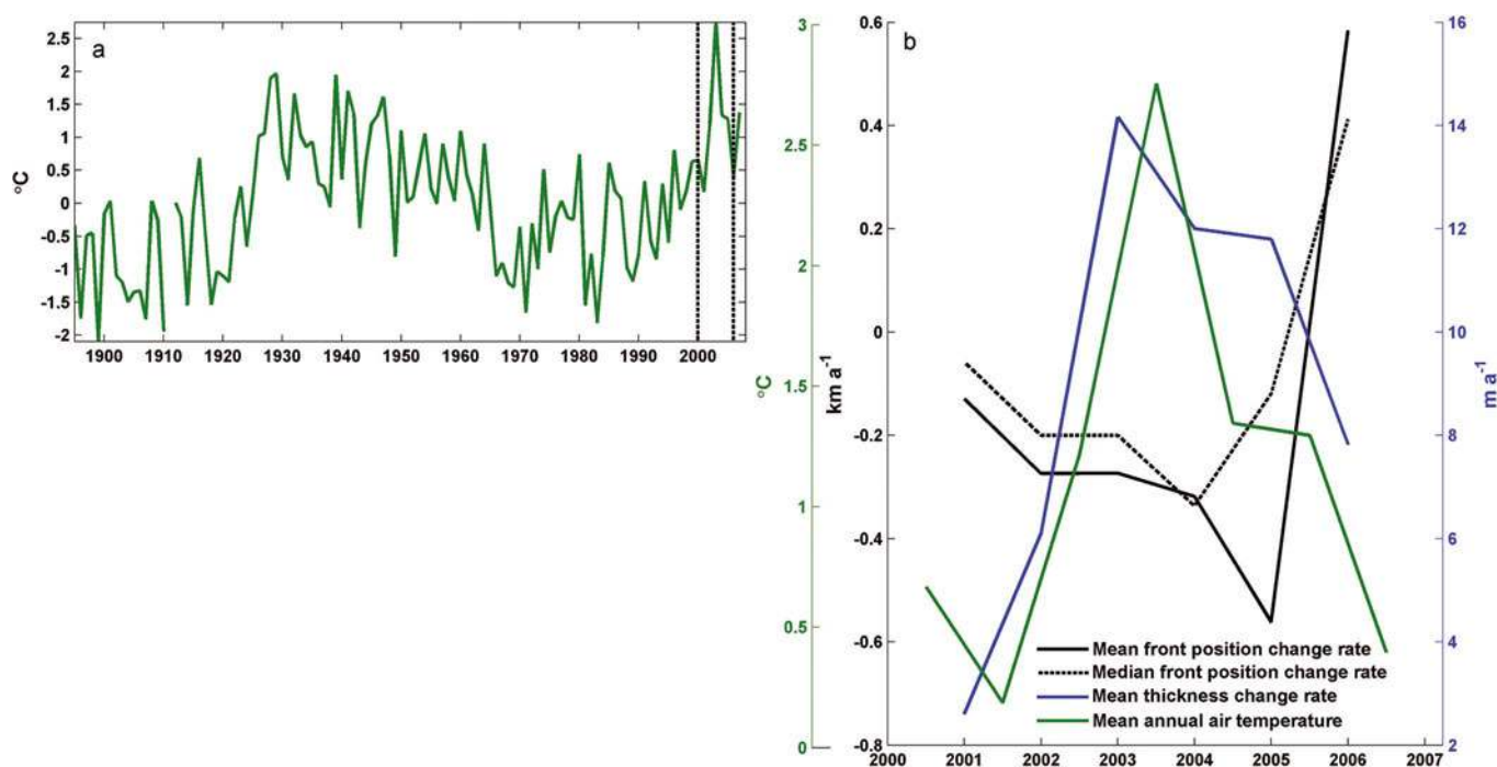
Fig. 10. (a) Plot of mean annual air-temperature anomaly recorded since 1895 at Anngmagssalik station, the location of which is shown in Figure 1. Dotted lines denote the time range of (b). (b) Plots of average and median change rates in front position (from Fig. 2; negative values indicate retreat), surface elevation (from Fig. 4) and mean annual air-temperature anomaly from the 114 year mean. The temperature dataset was obtained from the Goddard Institute for Space Studies ( http://data.giss.nasa.gov/gistemp/ ).
