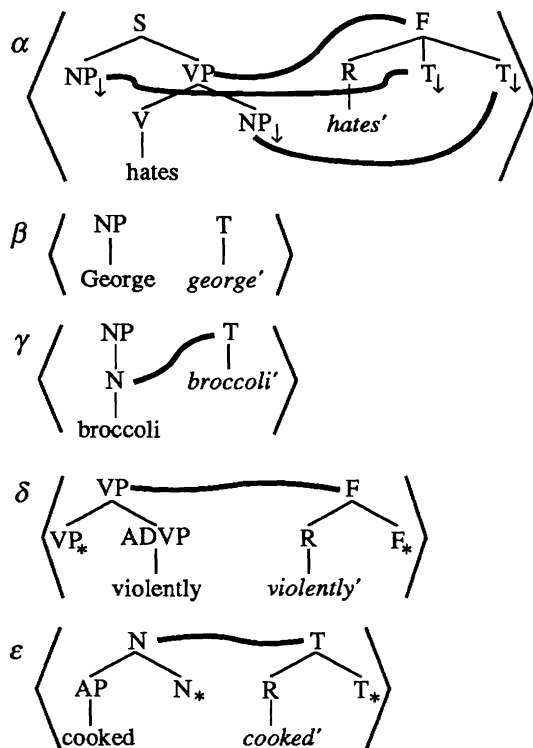
Figure 1: A sample synchronous TAG.
