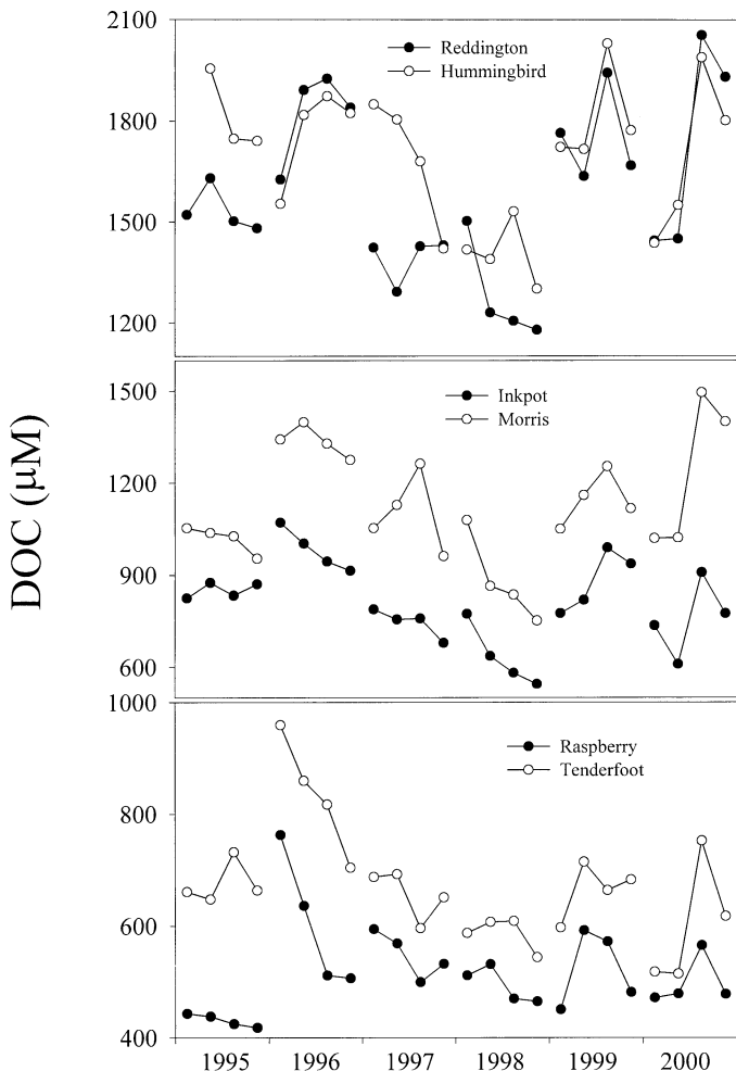
Fig. 2. Exemplary time series of DOC for pairs of lakes illustrating how synchrony was determined. Data are monthly values for May–August in each year. Correlations ( r ) for the pairs are: Reddington–Hummingbird, r = 0.69 , P = 0.001 ; Inkpot–Morris, r = 0.74 , P < 0.001 ; Raspberry–Tenderfoot, r = 0.71 , P < 0.001 .
