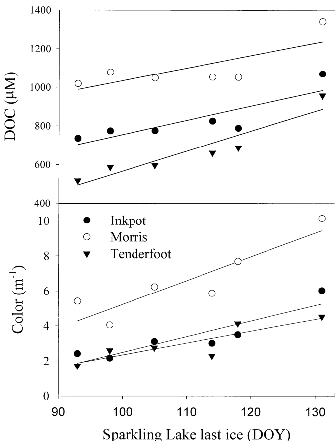
Fig. 5. Relationship between the May value of DOC or color for three of the study lakes and last date of complete ice cover on Sparkling Lake for the years 1995–2000. Symbols are Morris Lake (open circle), Inkpot Lake (closed circle), and Tenderfoot Lake (triangle). Data from Sparkling Lake provided by NTL-LTER.
