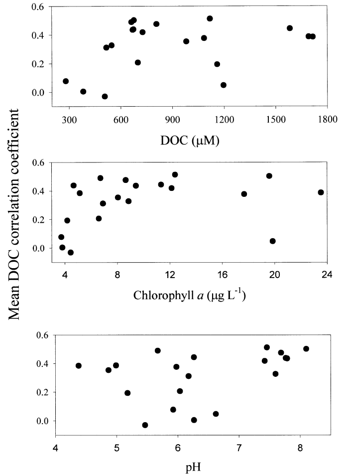
Fig. 4. Average DOC, chlorophyll, or pH versus the mean Pearson correlation coefficient for each lake. The mean DOC correlation of a lake is the average of 19 time series comparisons. Linear regressions for the mean correlation coefficient and DOC, chlorophyll, or pH were all not significant at P < 0.05 .
