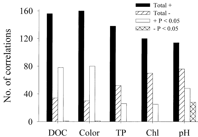
Fig. 3. Number of correlations that were positive (“total +,” filled bars), negative (“total −,” slashed bars), positive and significant ( P < 0.05 , open bars), negative and significant ( P < 0.05 , crosshatched bars) for DOC, color, total phosphorus (TP), chlorophyll a (Chl), and pH based on correlations between time series for each lake ( n = 190 ).
