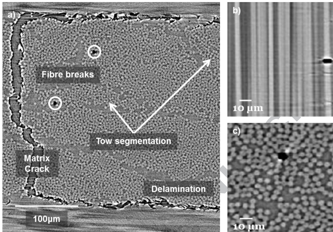
Figure 1: a) Cross-section of T700/M21 at the final load step (94% of final failure), showing fibre breaks in the 0^\circ ply, delamination, matrix crack due to 0^\circ splitting and tow segmentation. b) shows a fibre break with the loading direction being vertical, and (c) shows the same fibre break in a cross-section.
