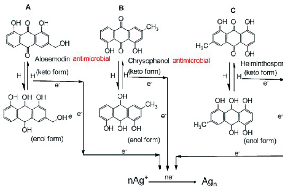
Figure 6 Possible mechanism of biosynthesis of Ag nanoparticles through quinone contained in fresh aloe vera extract
