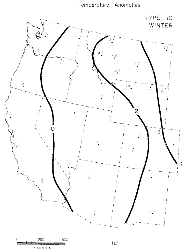
Figure 5. Seasonal temperature anomaly patterns for four circulation types: (a) Type 2, winter; (b) Type 7, winter; (c) Type 8, spring; (d) Type 10, winter
