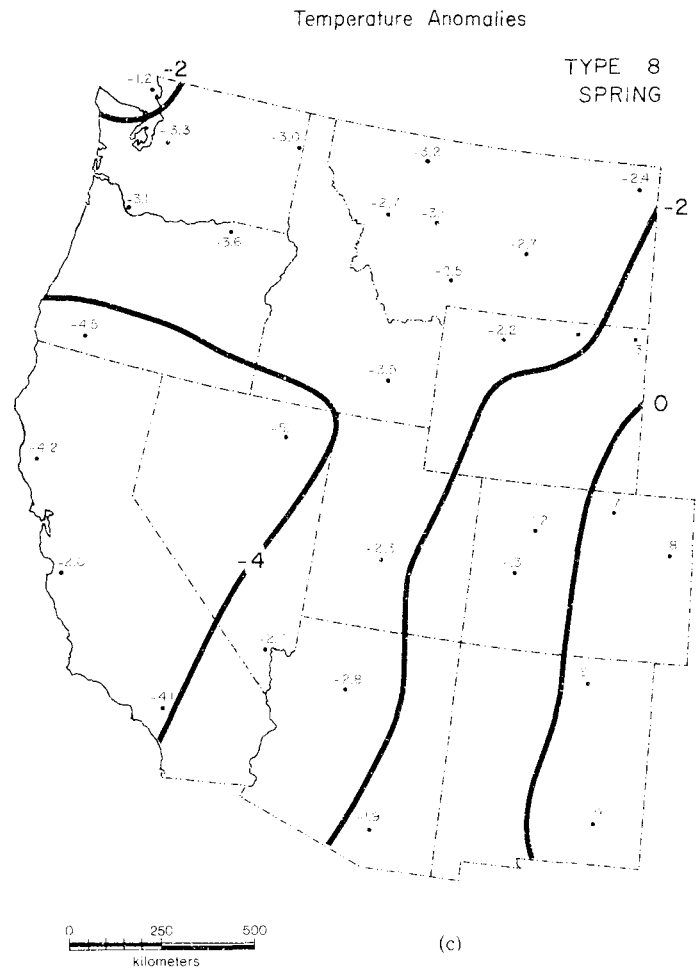
Figure 5. Seasonal temperature anomaly patterns for four circulation types: (a) Type 2, winter; (b) Type 7, winter; (c) Type 8, spring; (d) Type 10, winter
