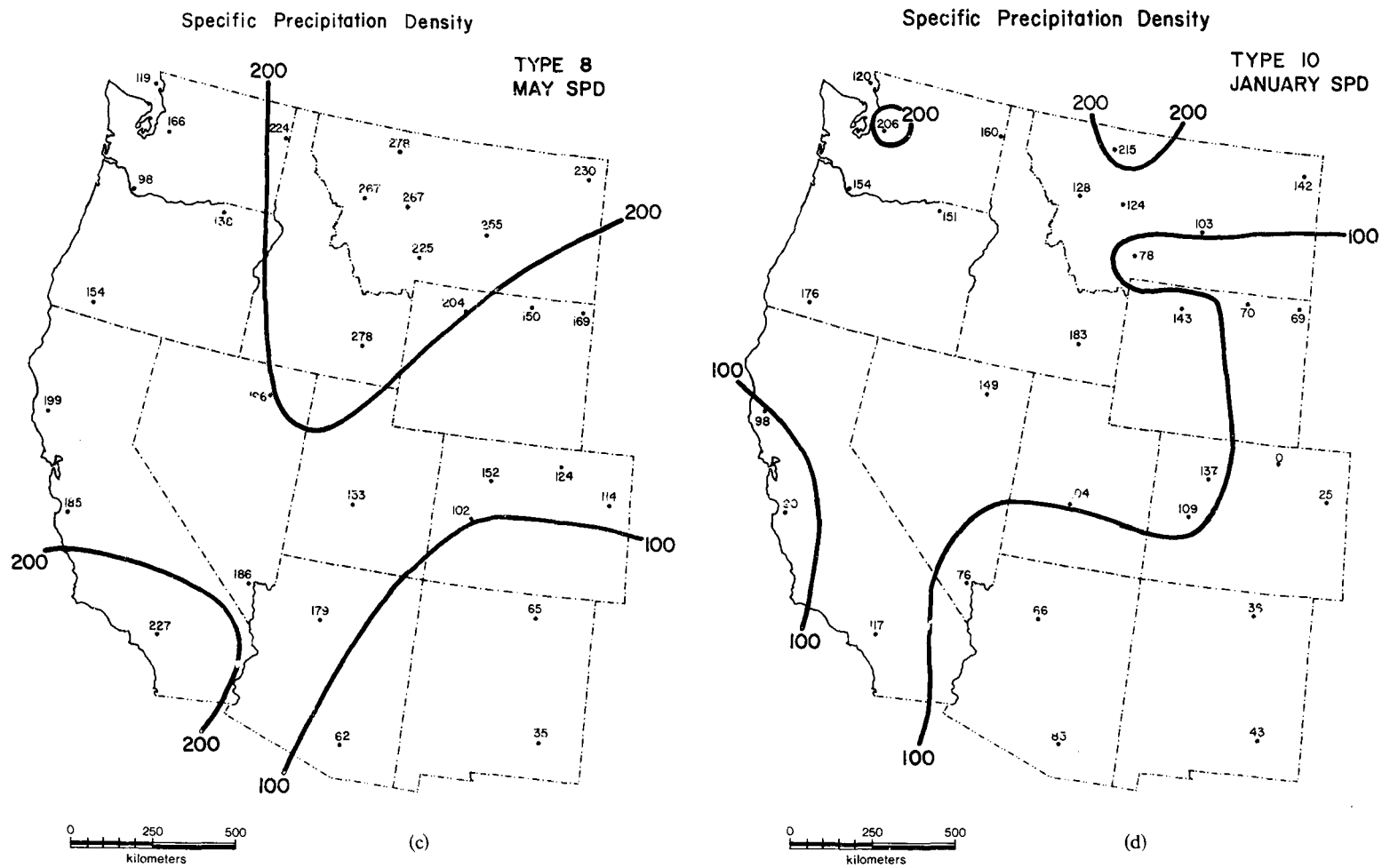
Figure 6. Seasonal patterns of specific precipitation density (see text) for four circulation types: (a) Type 2, January; (b) Type 7, January; (c) Type 8, May; (d) Type 10, January
