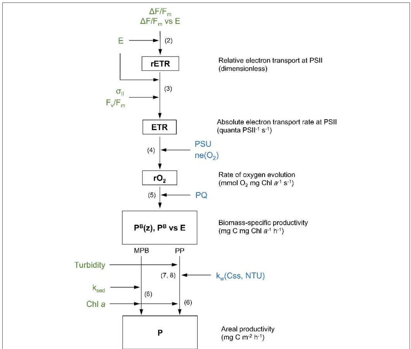
FIGURE 2 | Schematic describing the modeling workflow followed in this study. Biomass-specific productivity rates ( P^B , \text{mg C mg Chl a}^{-1} \text{h}^{-1} ) were calculated from irradiance (E) and fluorescence-based parameters ( F_v/F_m , \Delta F/F_m , \Delta F/F_m , \sigma_{II} ). Productivity per unit area was calculated by depth-integrating P^B using light-response curves of P^B , chlorophyll a content, and light attenuation. Depth-integration was carried out differently for phytoplankton (PP) and microphytobenthos (MPB), using light attenuation coefficient for the water column ( k_w ) and the sediment ( k_s ), respectively. Parameters in green were measured in this study. Parameters in blue were taken from published sources. Numbers represent the equations describing each step.
