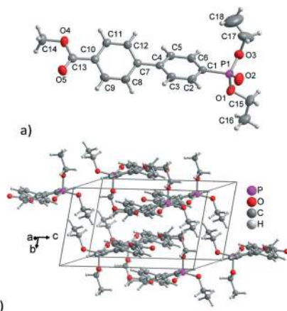
Fig. 2 (a) Asymmetric unit (50% thermal ellipsoids) and (b) crystal packing in 3 . Selected distances ( \text{\AA} ) and angles ( ^\circ ): P1–O1 1.560(2), P1–O2 1.462(2), P1–O3 1.567(2), C13–O5 1.195(3), C13–O4 1.341(3), O1–P1–O2 116.11(13), O2–P1–O3 113.98(13), O1–P1–O3 102.44(13).
